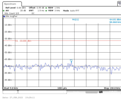
Band2-15MHz-16QAM-19125-1RB#0-Range1:0.009~0.15MHz
