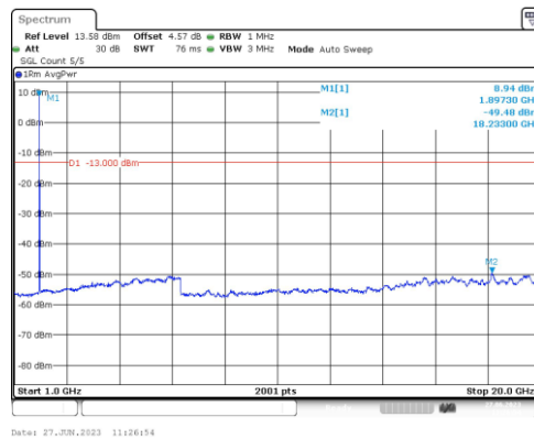
Band2-10MHz-16QAM-19150-1RB#0-Range4:1000~20000MHz
