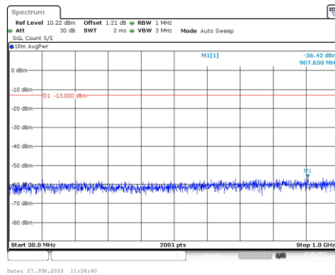
Band2-10MHz-16QAM-19150-1RB#0-Range3:30~1000MHz
