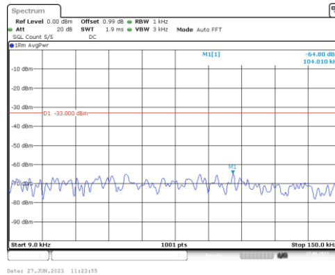
Band2-10MHz-QPSK-18900-1RB#0-Range1:0.009~0.15MHz
