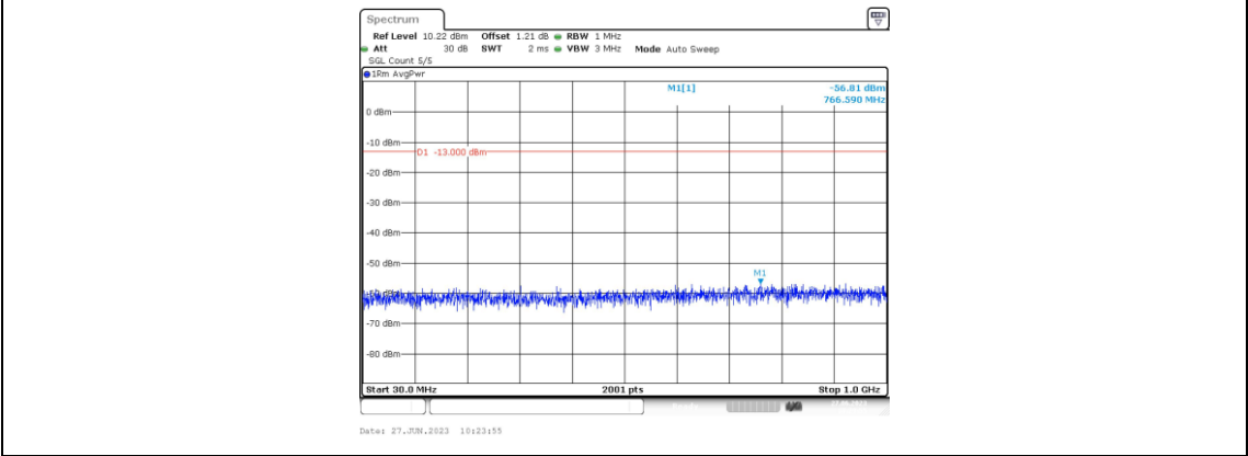
Band2-3MHz-16QAM-19185-1RB#0-Range3:30~1000MHz
