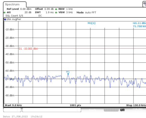
Band2-15MHz-QPSK-18675-1RB#0-Range1:0.009~0.15MHz
