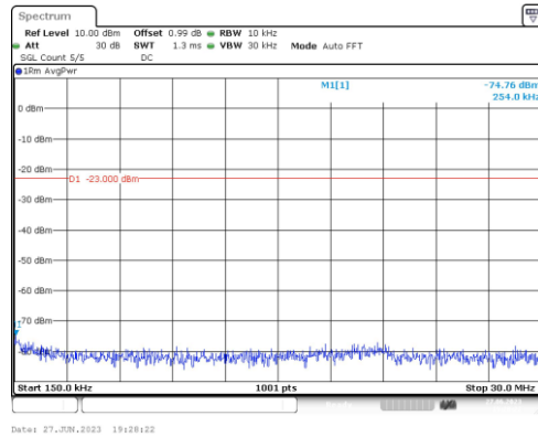
Band2-15MHz-16QAM-19125-1RB#0-Range2:0.15~30MHz
