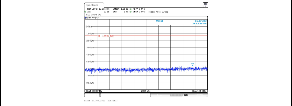
Band4-1.4MHz-QPSK-20393-1RB#0-Range3:30~1000MHz
