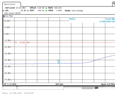
Band4-20MHz-16QAM-20050-1RB#0
