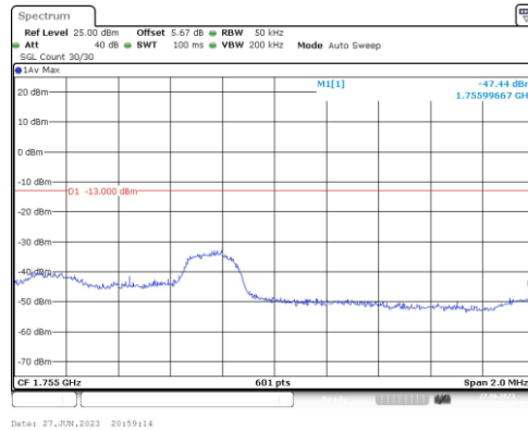
Band4-3MHz-16QAM-20385-1RB#0
