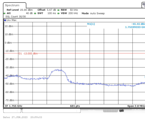
Band4-3MHz-QPSK-20385-1RB#0
