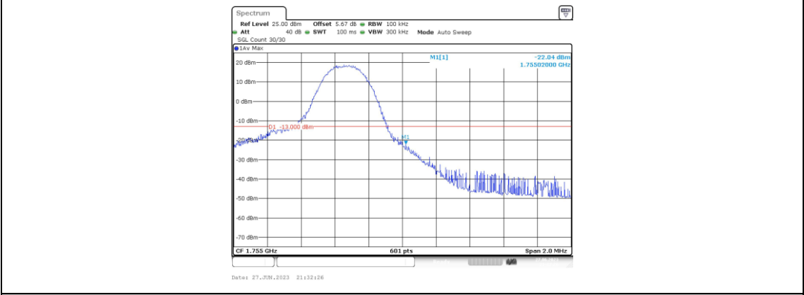
Band4-5MHz-16QAM-20375-1RB#24
