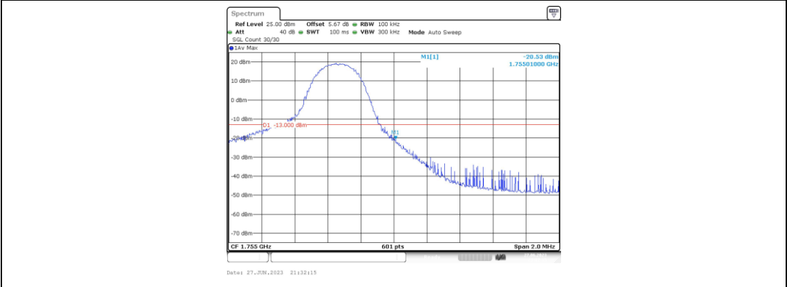
Band4-5MHz-QPSK-20375-1RB#24
