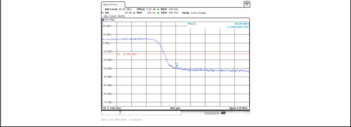
Band4-5MHz-16QAM-20375-1RB#24
