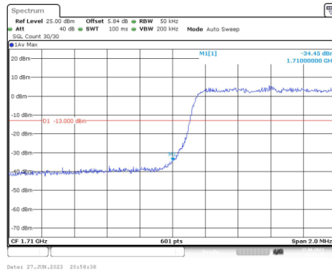
Band4-3MHz-16QAM-19965-15RB#0
