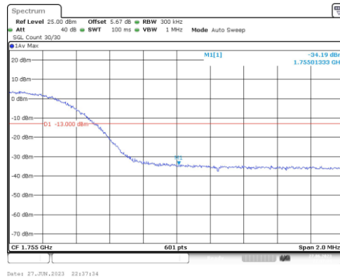
Band4-15MHz-16QAM-20325-75RB#0
