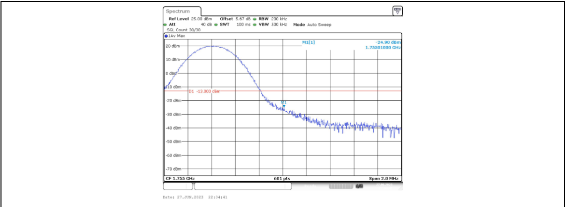
Band4-10MHz-16QAM-20350-1RB#49
