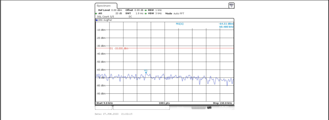
Band4-3MHz-QPSK-20175-1RB#0-Range1:0.009~0.15MHz
