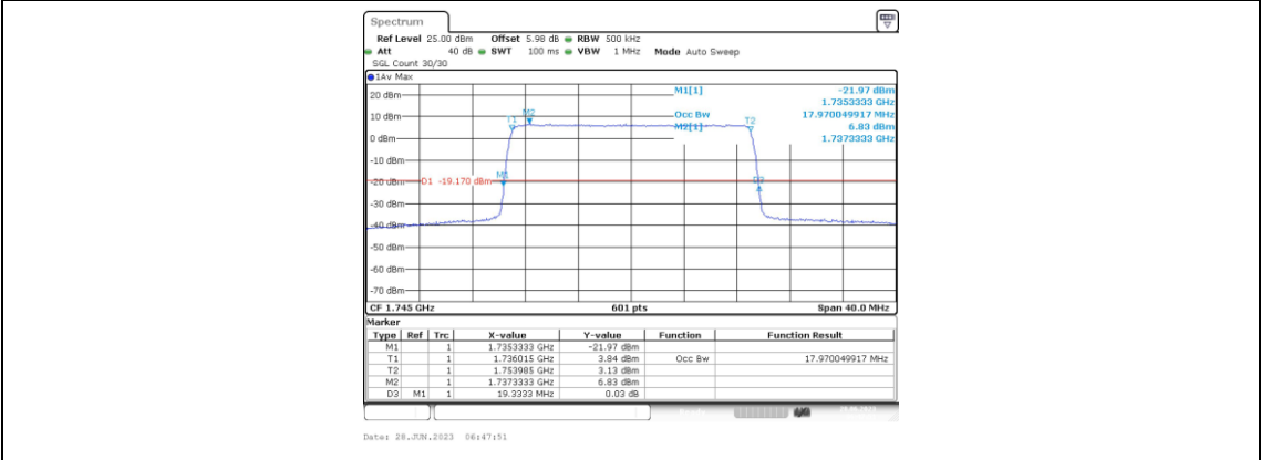
Band66-20MHz-QPSK-132322-100RB#0-17.97
