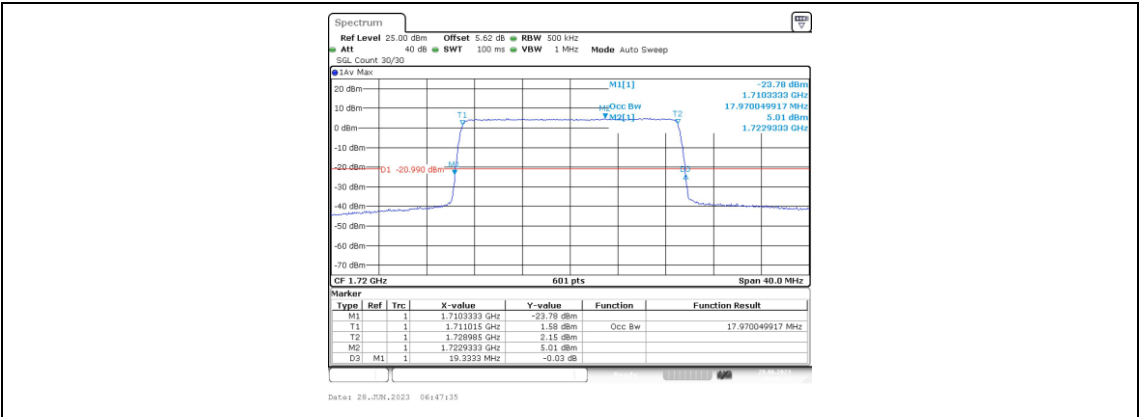
Band66-20MHz-16QAM-132072-100RB#0-17.97
