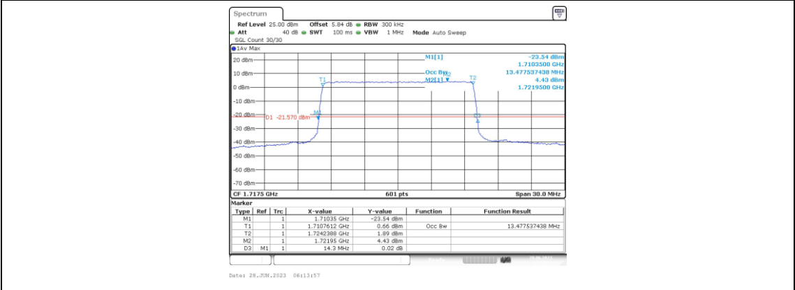
Band66-15MHz-16QAM-132047-75RB#0-13.478
