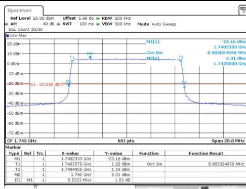
Band66-10MHz-QPSK-132322-50RB#0-8.985
