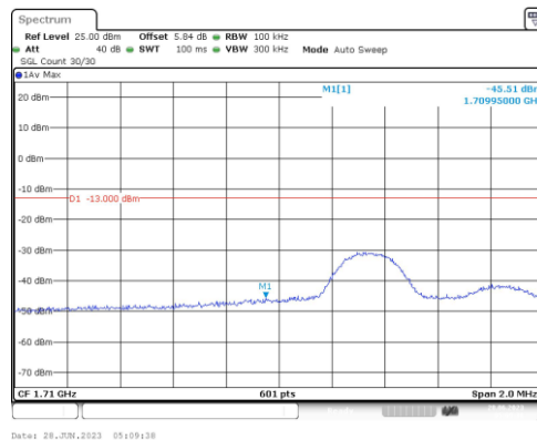
Band66-5MHz-QPSK-131997-1RB#24
