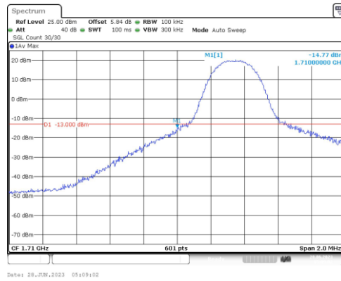
Band66-5MHz-QPSK-131997-1RB#0
