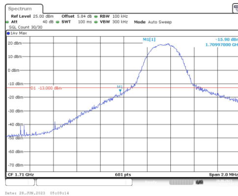
Band66-5MHz-16QAM-131997-1RB#0
