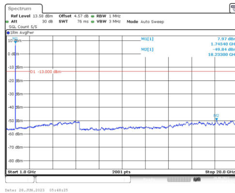
Band66-10MHz-16QAM-132322-1RB#0-Range4:1000~20000MHz
