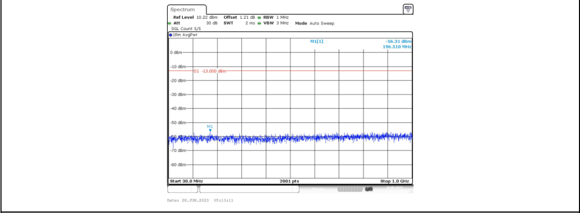
Band66-5MHz-16QAM-131997-1RB#0-Range3:30~1000MHz
