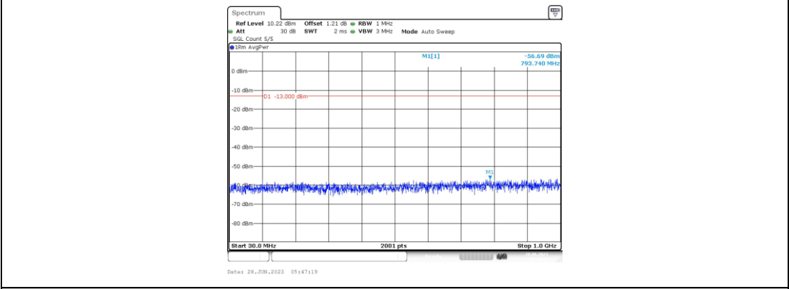
Band66-10MHz-QPSK-132322-1RB#0-Range3:30~1000MHz
