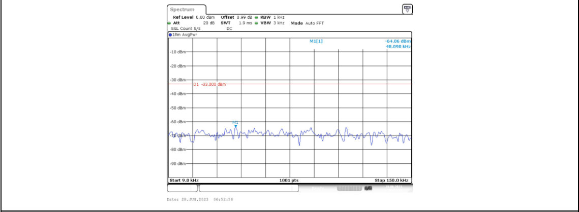
Band66-20MHz-16QAM-132072-1RB#0-Range1:0.009~0.15MHz
