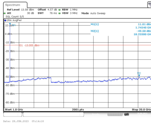
Band66-5MHz-QPSK-132322-1RB#0-Range4:1000~20000MHz
