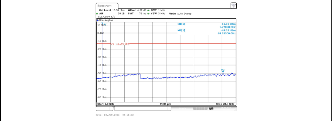
Band66-5MHz-QPSK-132647-1RB#0-Range4:1000~20000MHz
