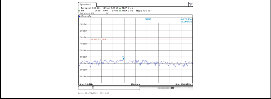
Band66-5MHz-16QAM-132647-1RB#0-Range1:0.009~0.15MHz
