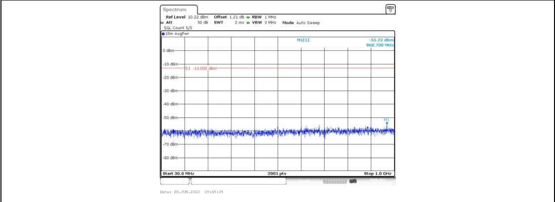
Band66-10MHz-QPSK-132022-1RB#0-Range3:30~1000MHz
