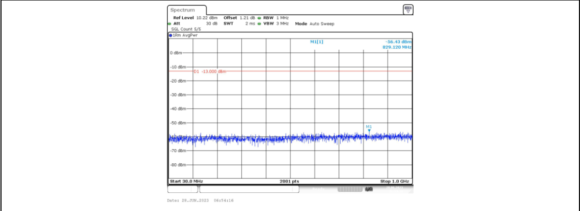
Band66-20MHz-QPSK-132322-1RB#0-Range3:30~1000MHz
