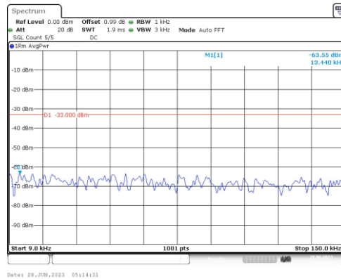
Band66-5MHz-16QAM-132322-1RB#0-Range1:0.009~0.15MHz
