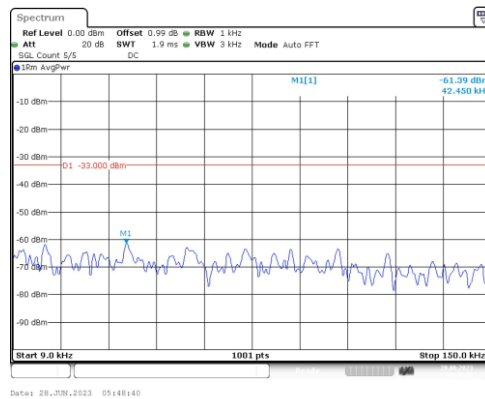
Band66-10MHz-QPSK-132622-1RB#0-Range1:0.009~0.15MHz
