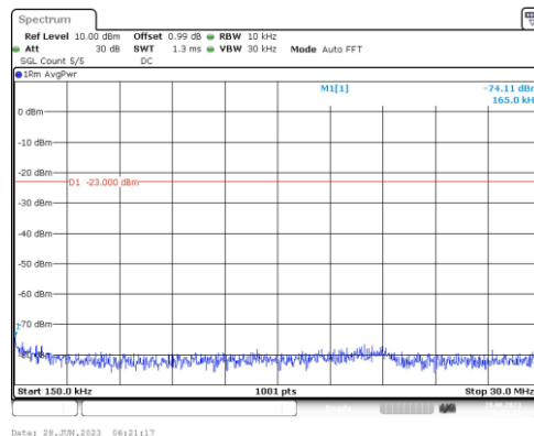
Band66-15MHz-16QAM-132322-1RB#0-Range2:0.15~30MHz
