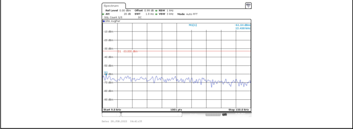
Band66-3MHz-QPSK-132657-1RB#0-Range1:0.009~0.15MHz
