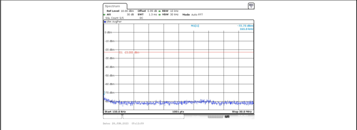
Band66-5MHz-16QAM-131997-1RB#0-Range2:0.15~30MHz
