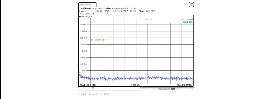
Band66-10MHz-QPSK-132322-1RB#0-Range2:0.15~30MHz
