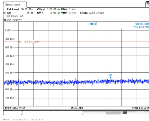
Band66-15MHz-16QAM-132322-1RB#0-Range3:30~1000MHz
