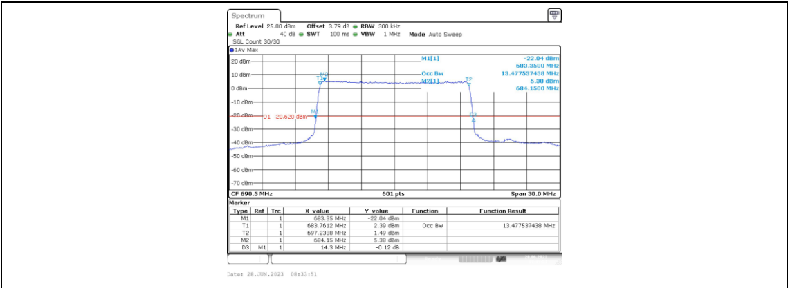
Band71-15MHz-16QAM-133397-75RB#0-13.478
