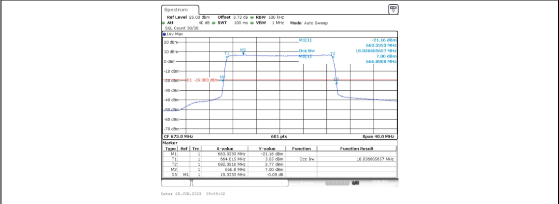
Band71-20MHz-QPSK-133222-100RB#0-18.037
