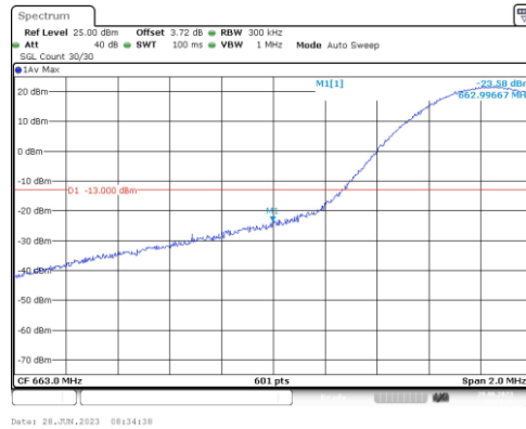
Band71-15MHz-16QAM-133197-1RB#0
