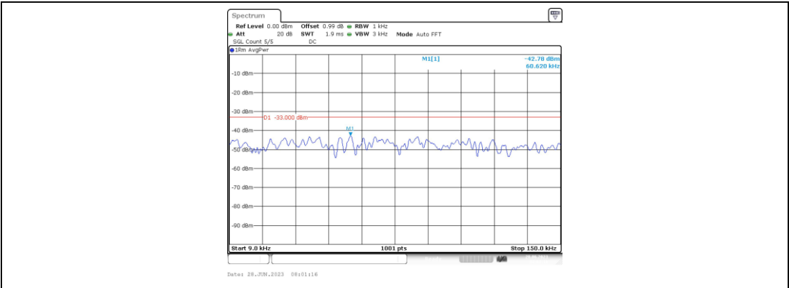
Band71-10MHz-QPSK-133172-1RB#0-Range1:0.009~0.15MHz
