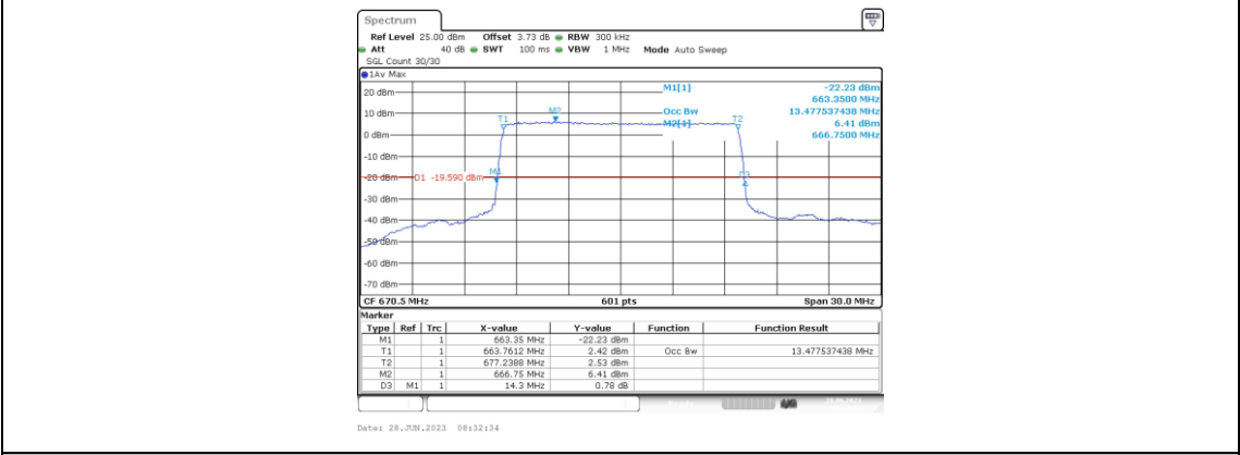
Band71-15MHz-QPSK-133197-75RB#0-13.478
