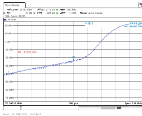
Band71-15MHz-QPSK-133197-1RB#0
