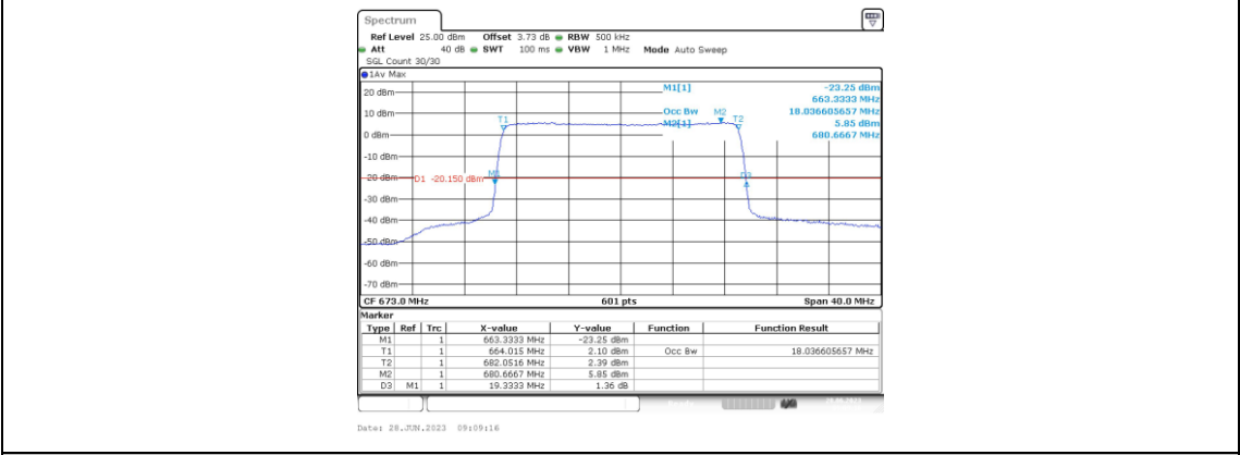
Band71-20MHz-16QAM-133222-100RB#0-18.037
