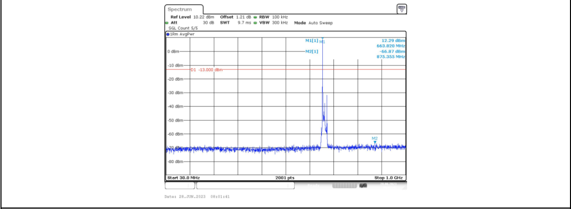
Band71-10MHz-QPSK-133172-1RB#0-Range3:30~1000MHz
