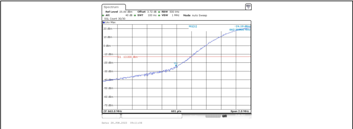
Band71-20MHz-16QAM-133222-1RB#0
