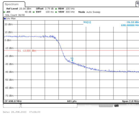
Band71-5MHz-16QAM-133447-25RB#0
