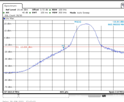
Band71-5MHz-16QAM-133147-1RB#0
