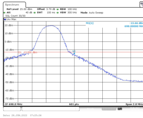
Band71-5MHz-16QAM-133447-1RB#24
