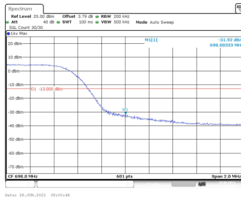
Band71-10MHz-16QAM-133422-50RB#0
