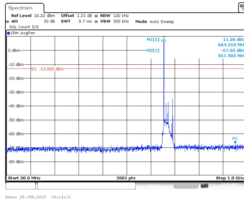
Band71-20MHz-QPSK-133222-1RB#0-Range3:30~1000MHz
