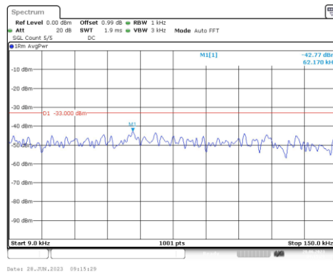
Band71-20MHz-QPSK-133322-1RB#0-Range1:0.009~0.15MHz
