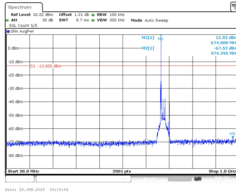
Band71-20MHz-QPSK-133322-1RB#0-Range3:30~1000MHz
