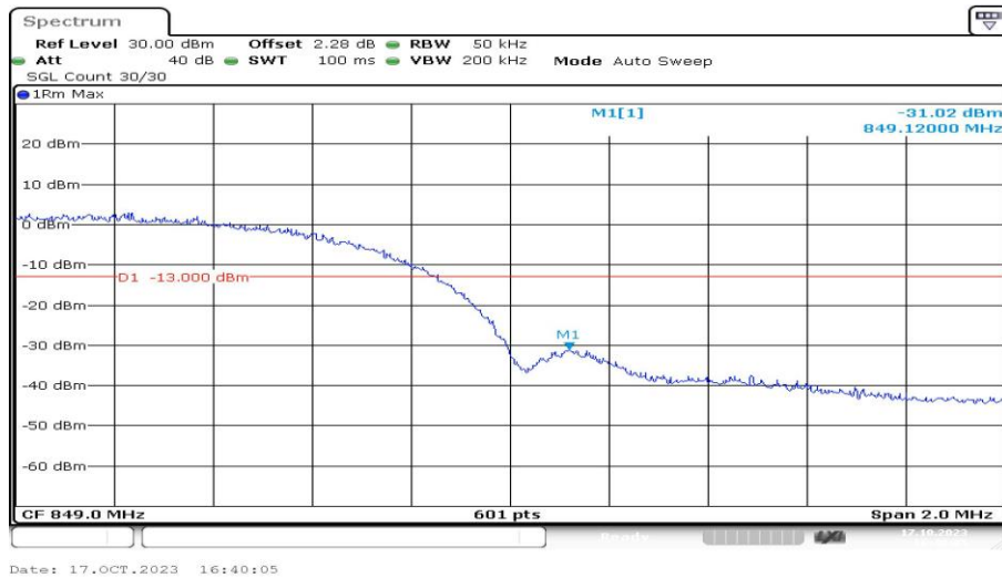
Band5-4233-3-PASS
