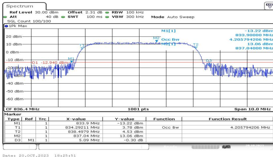
Band5-4182-3-PASS
