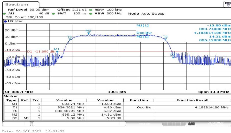
Band5-4182-5-PASS
