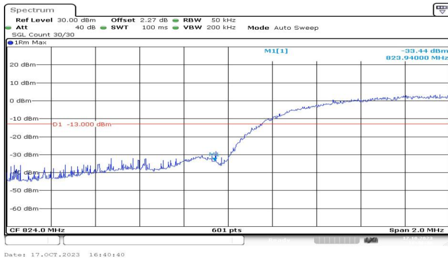
Band5-4132-4-PASS
