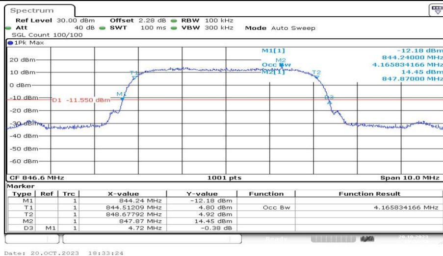
Band5-4233-5-PASS
