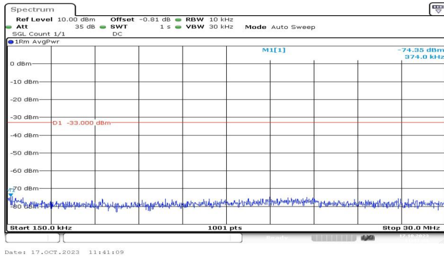
Band4-1513-2-0.15~30MHz-PASS
