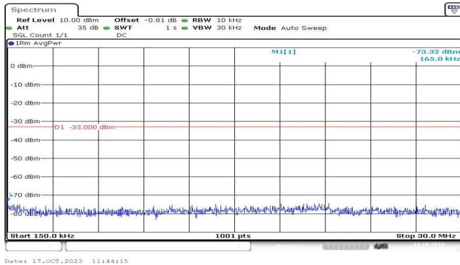
Band4-1513-3-0.15~30MHz-PASS
