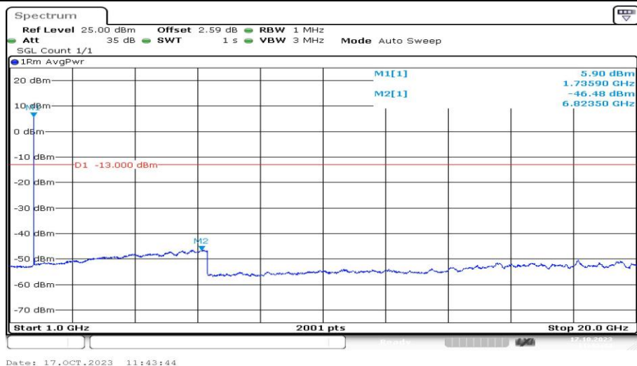
Band4-1413-3-1000~20000MHz-PASS
