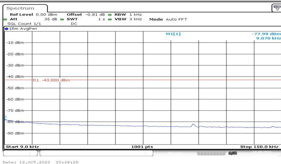
Band2-9538-4-0.009~0.15MHz-PASS
