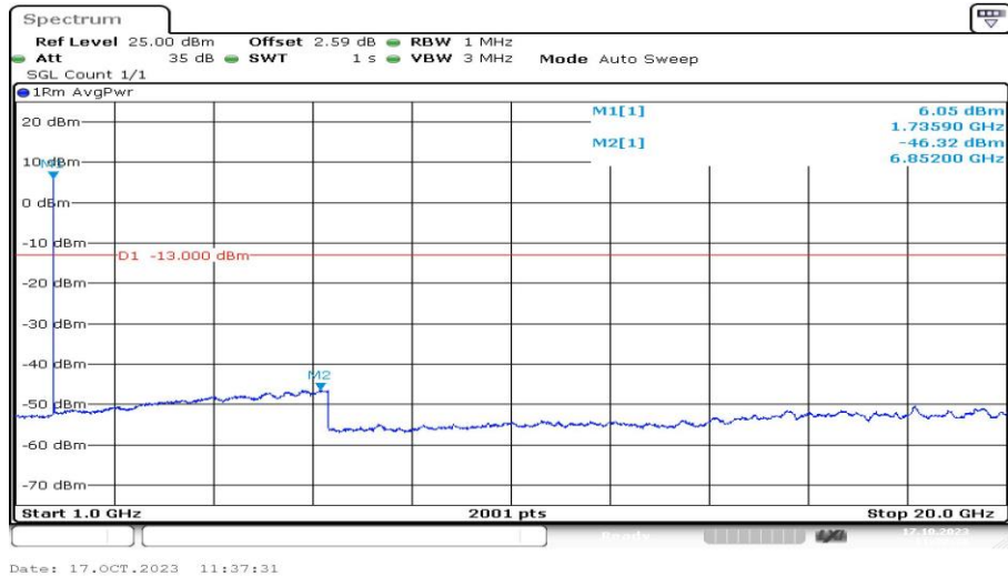
Band4-1413-1-1000~20000MHz-PASS
