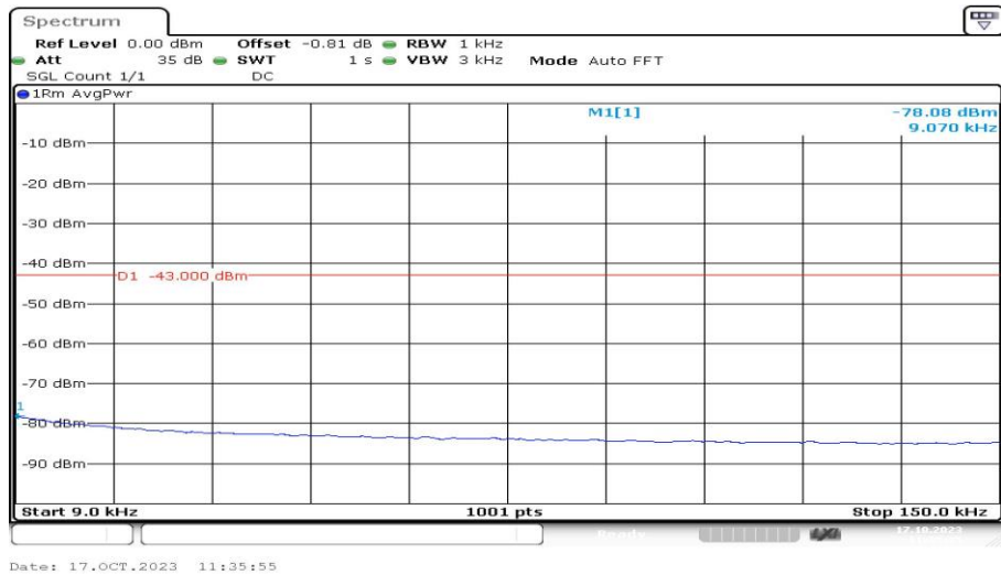
Band4-1312-1-0.009~0.15MHz-PASS
