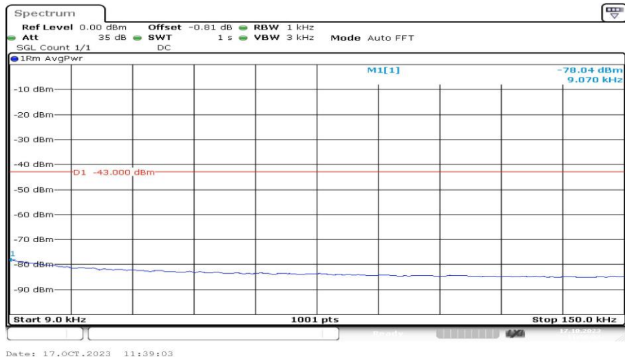
Band4-1312-2-0.009~0.15MHz-PASS
