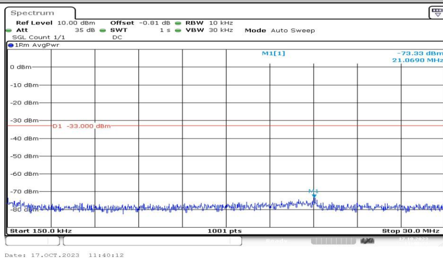
Band4-1413-2-0.15~30MHz-PASS
