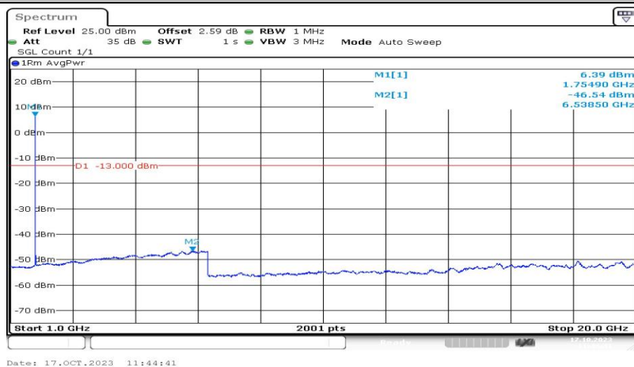
Band4-1513-3-1000~20000MHz-PASS
