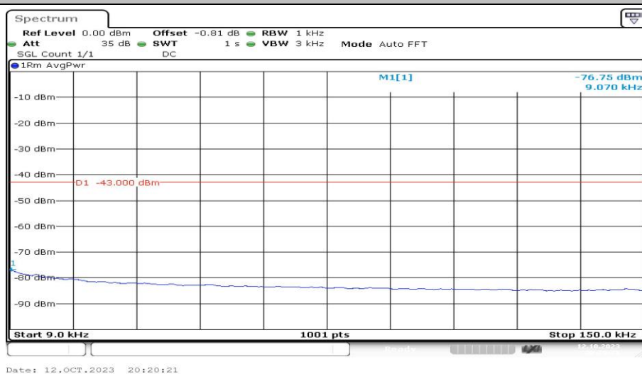
Band2-9538-2-0.009~0.15MHz-PASS
