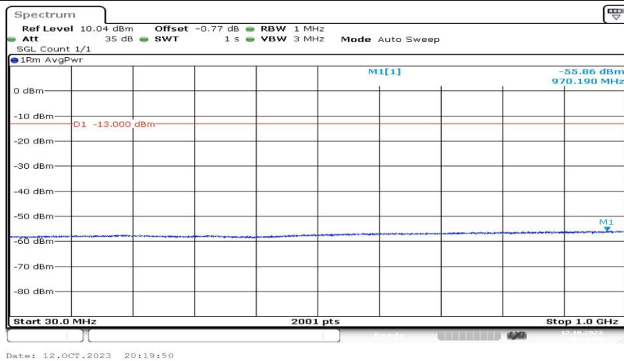
Band2-9400-2-30~1000MHz-PASS
