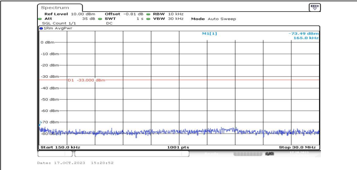
Band4-1513-2-0.15~30MHz-PASS
