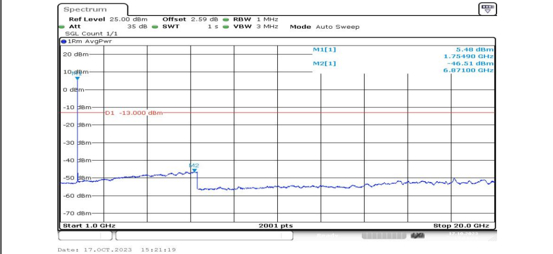
Band4-1513-2-1000~20000MHz-PASS
