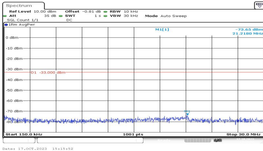
Band4-1513-1-0.15~30MHz-PASS
