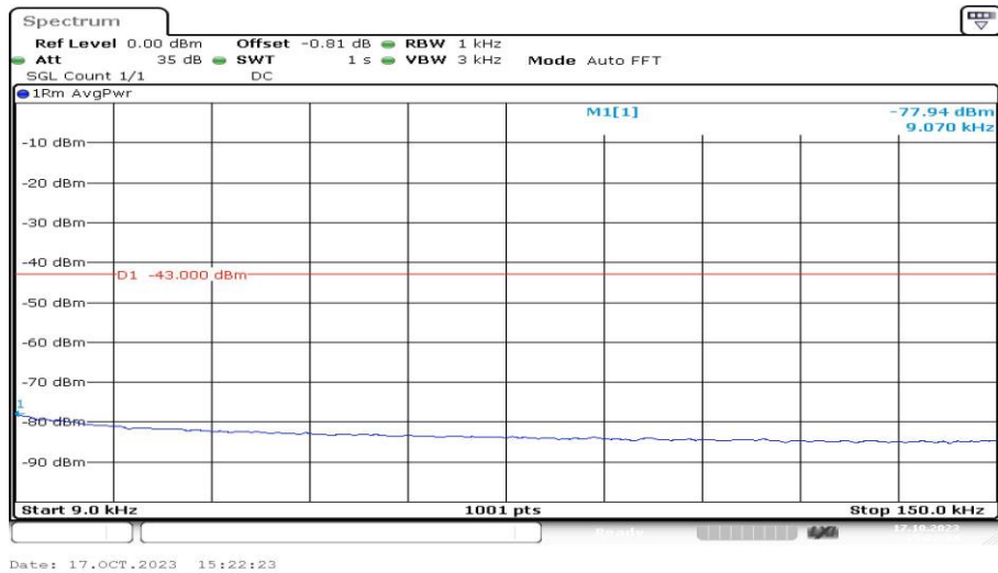
Band4-1312-3-0.009~0.15MHz-PASS
