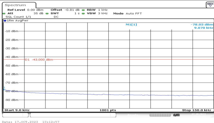
Band2-9262-4-0.009~0.15MHz-PASS
