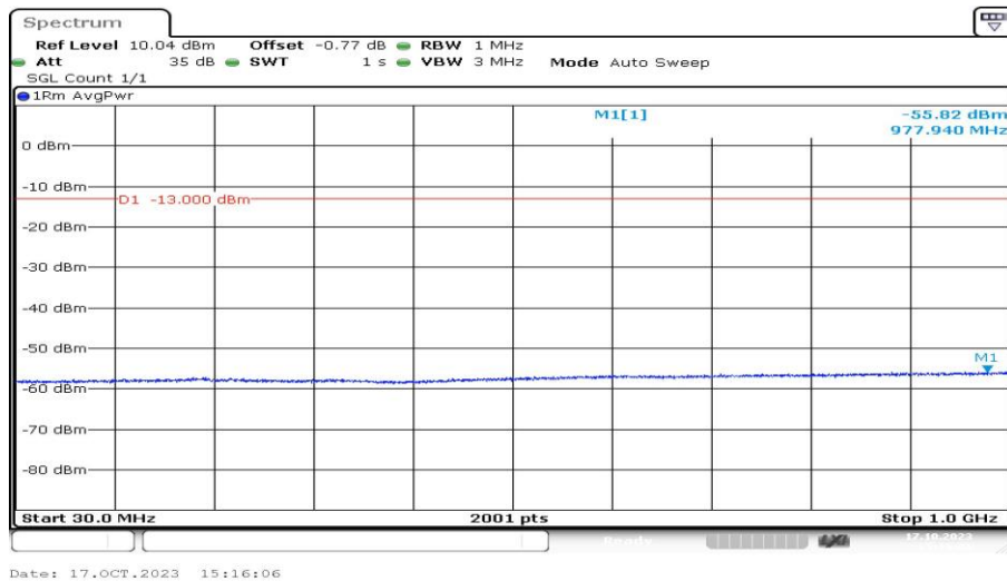
Band4-1513-1-30~1000MHz-PASS
