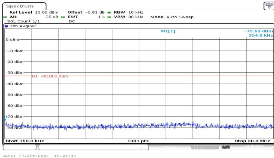
Band4-1312-3-0.15~30MHz-PASS
