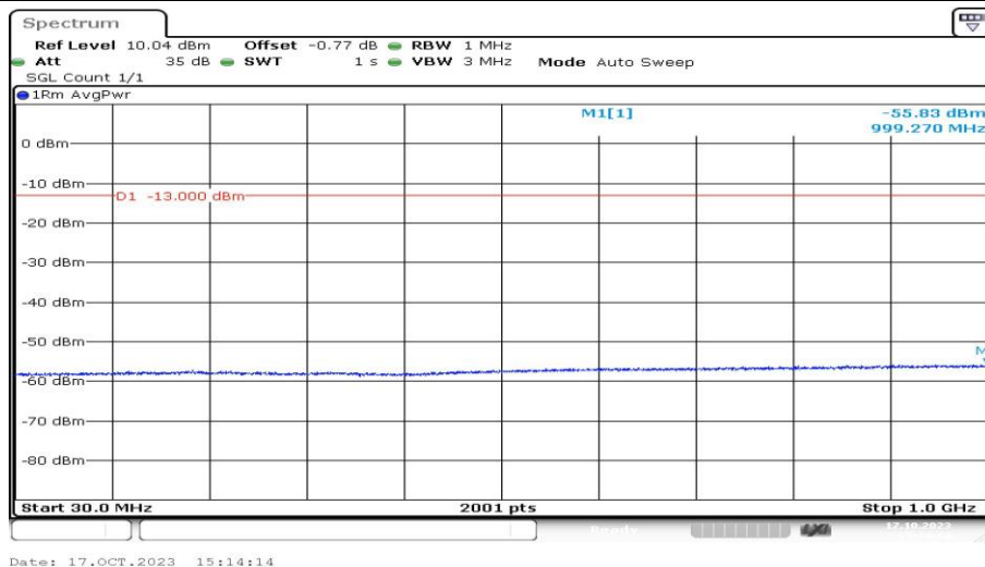
Band4-1413-1-30~1000MHz-PASS
