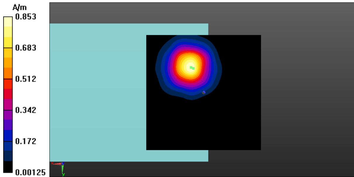
Fig A.10 T-Coil LTE-Band 66-Z
