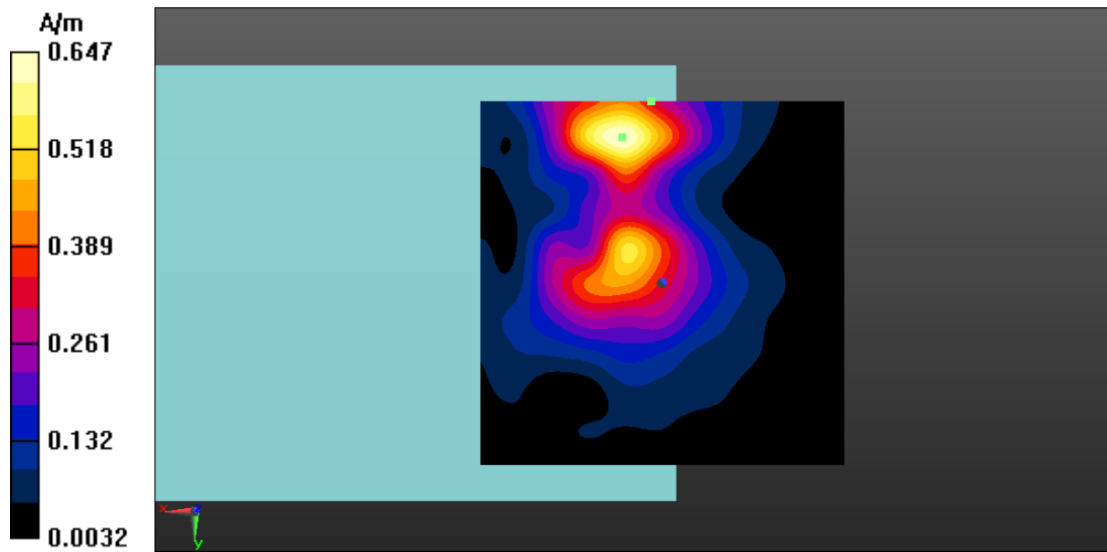
Fig A.18 T-Coil WCDMA Band 4-Y
