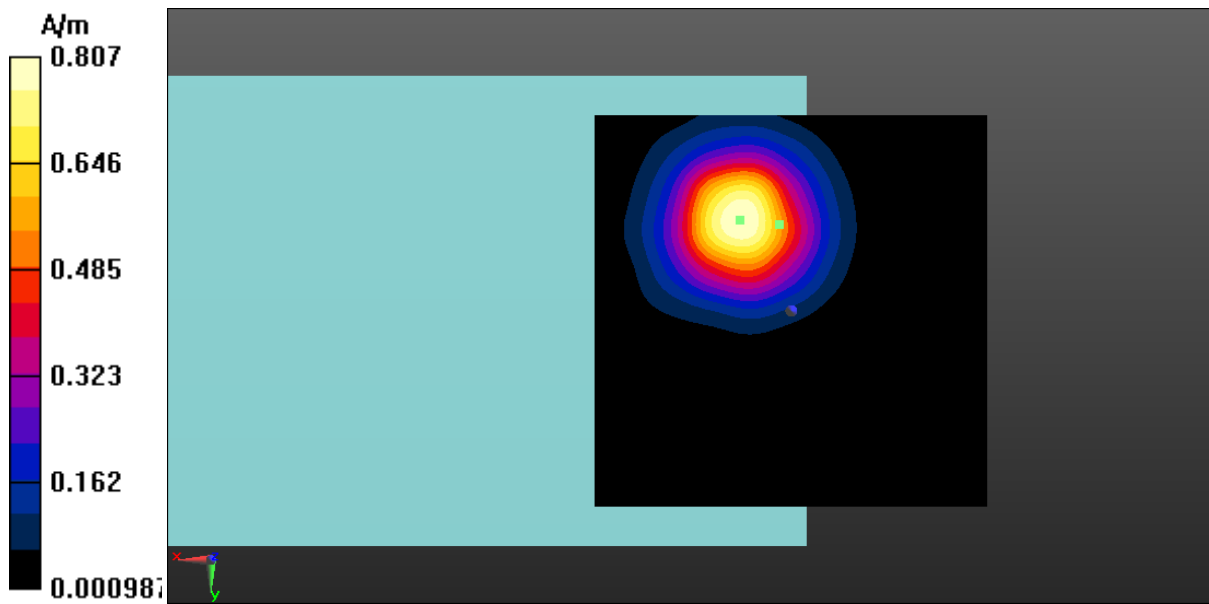
Fig A.11 T-Coil LTE-Band 71-Z
