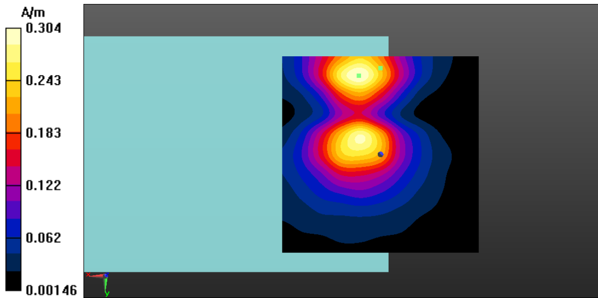
Fig A.11 T-Coil LTE-Band 71-Y
