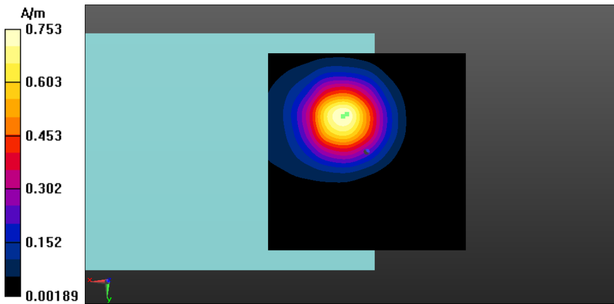
Fig A.16 T-Coil WLAN 5.2GHz-Z
