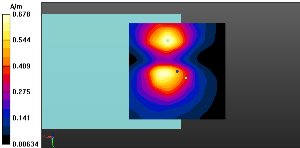
Fig A.23 T-Coil WLAN 2.4GHz-Y
