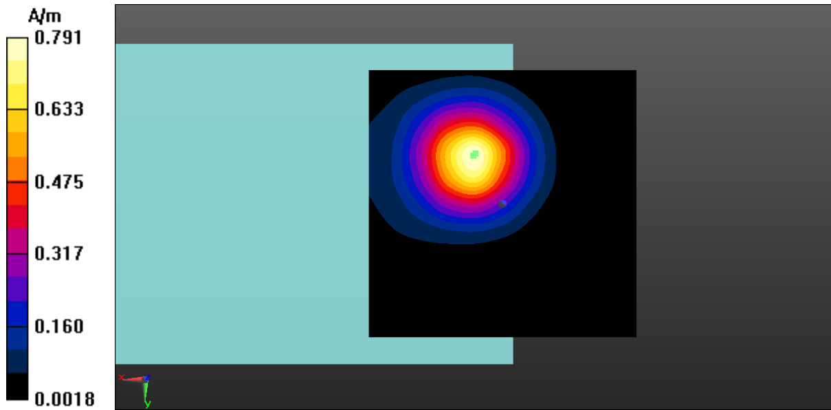
Fig A.18 T-Coil WLAN 5.5GHz-Z
