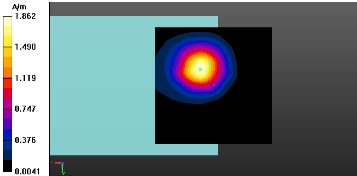
Fig A.22 T-Coil LTE-Band 41-Z
