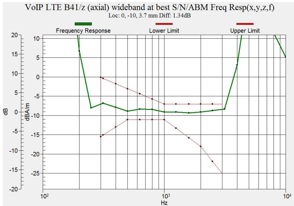
Figure B.22 Frequency Response of LTE Band 41 (Google Meet)
