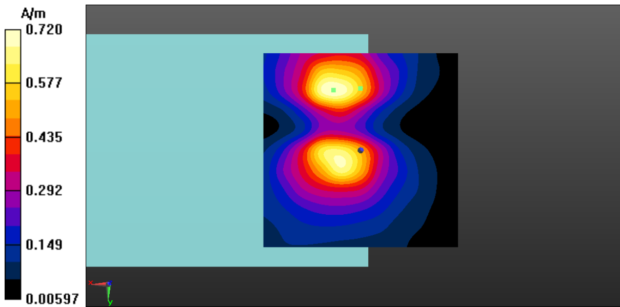
Fig A.22 T-Coil LTE-Band 41-Y
