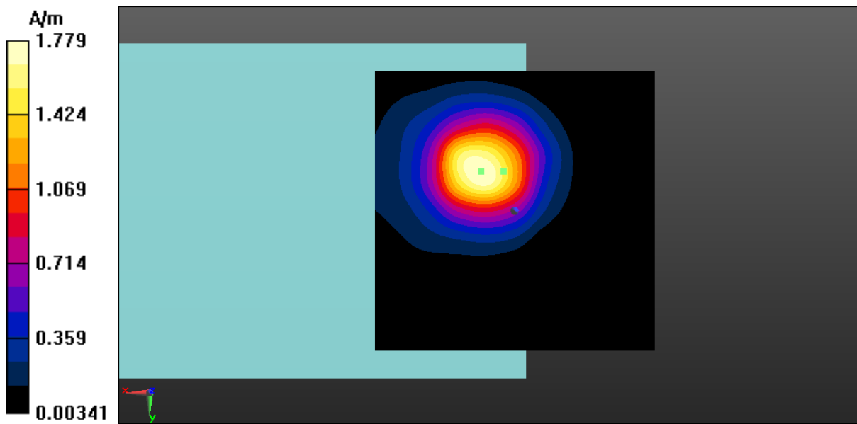
Fig A.23 T-Coil WLAN 2.4GHz-Z
