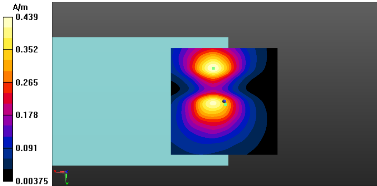
Fig A.11 T-Coil LTE-Band 17-Y
