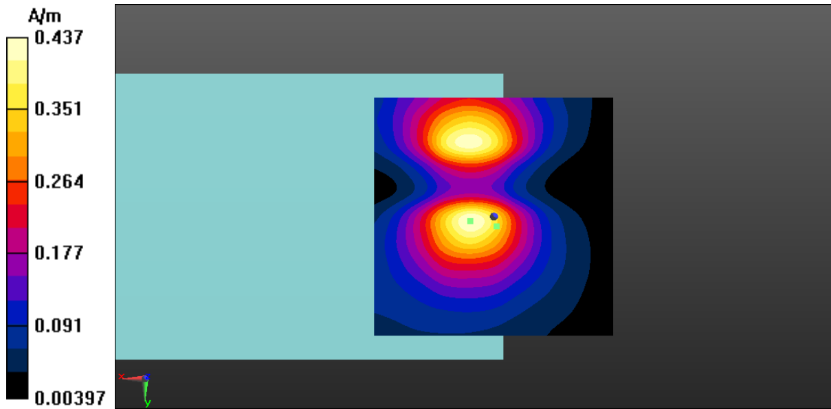
Fig A.14 T-Coil LTE-Band 41-Y
