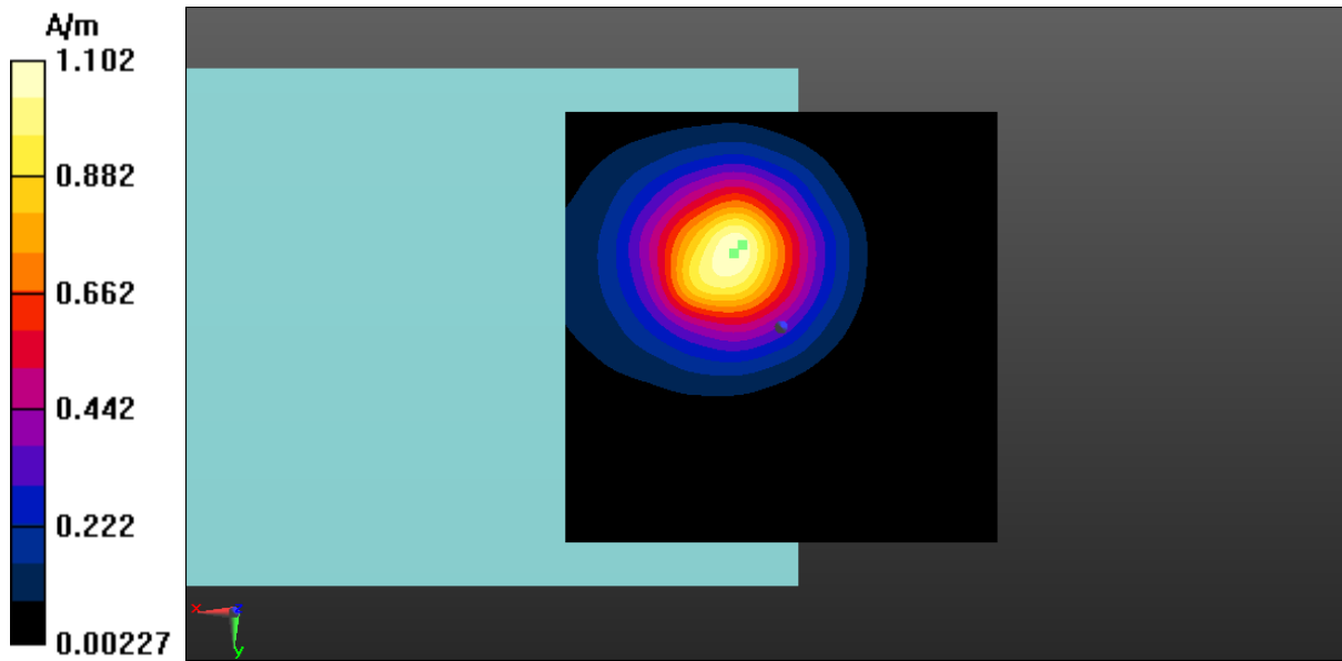
Fig A.19 T-Coil WLAN 5.8GHz-Z
