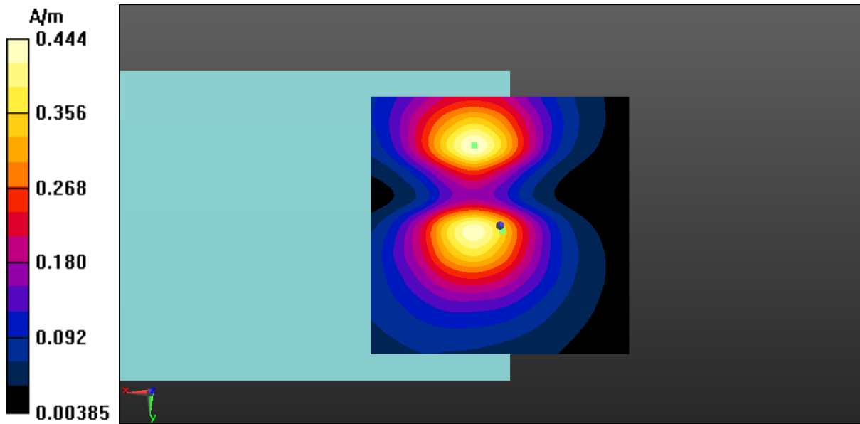
Fig A.10 T-Coil LTE-Band 13-Y
