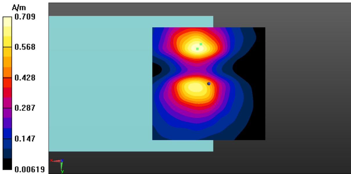
Fig A.21 T-Coil WCDMA Band 4-Y
