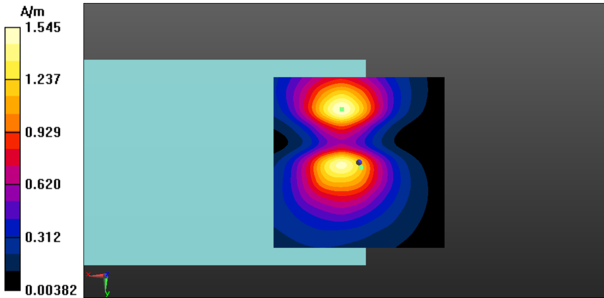
Fig A.9 T-Coil LTE-Band 12-Y
