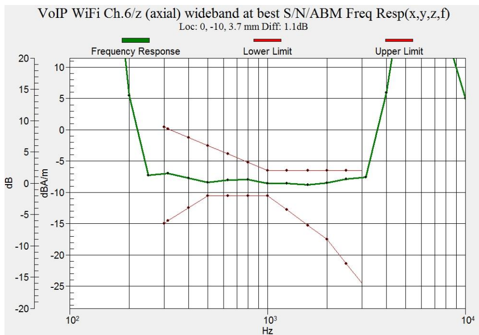
Figure B.23 Frequency Response of WLAN 2.4GHz (Google Meet)
