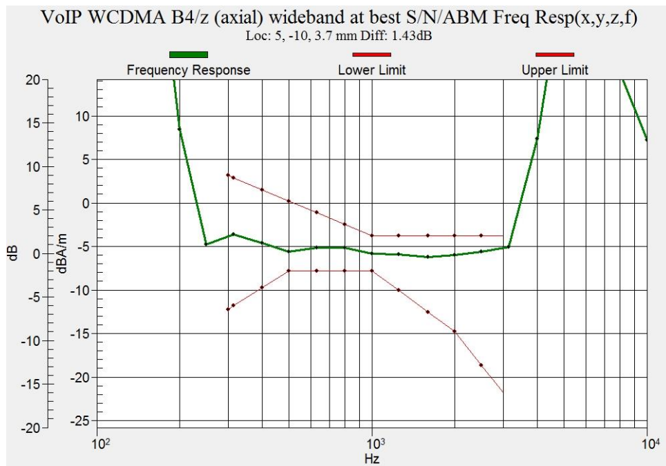
Figure B.21 Frequency Response of WCDMA Band 4 (Google Meet)
