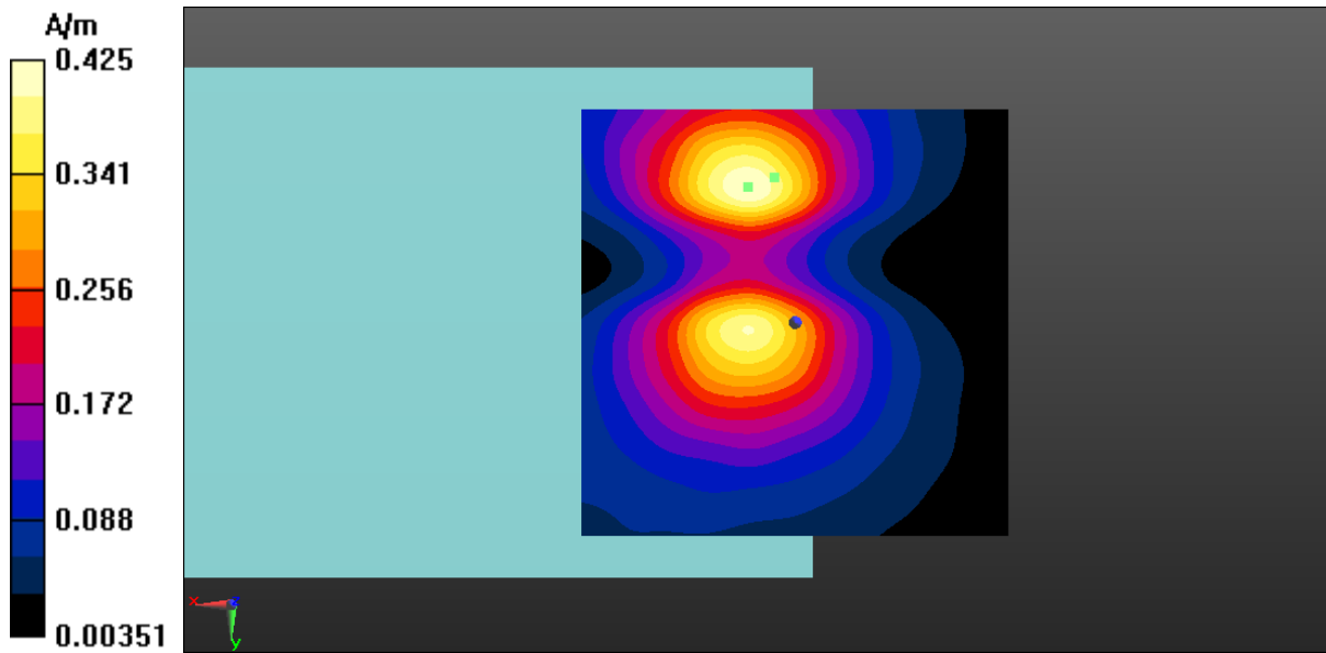
Fig A.19 T-Coil WLAN 5.8GHz-Y
