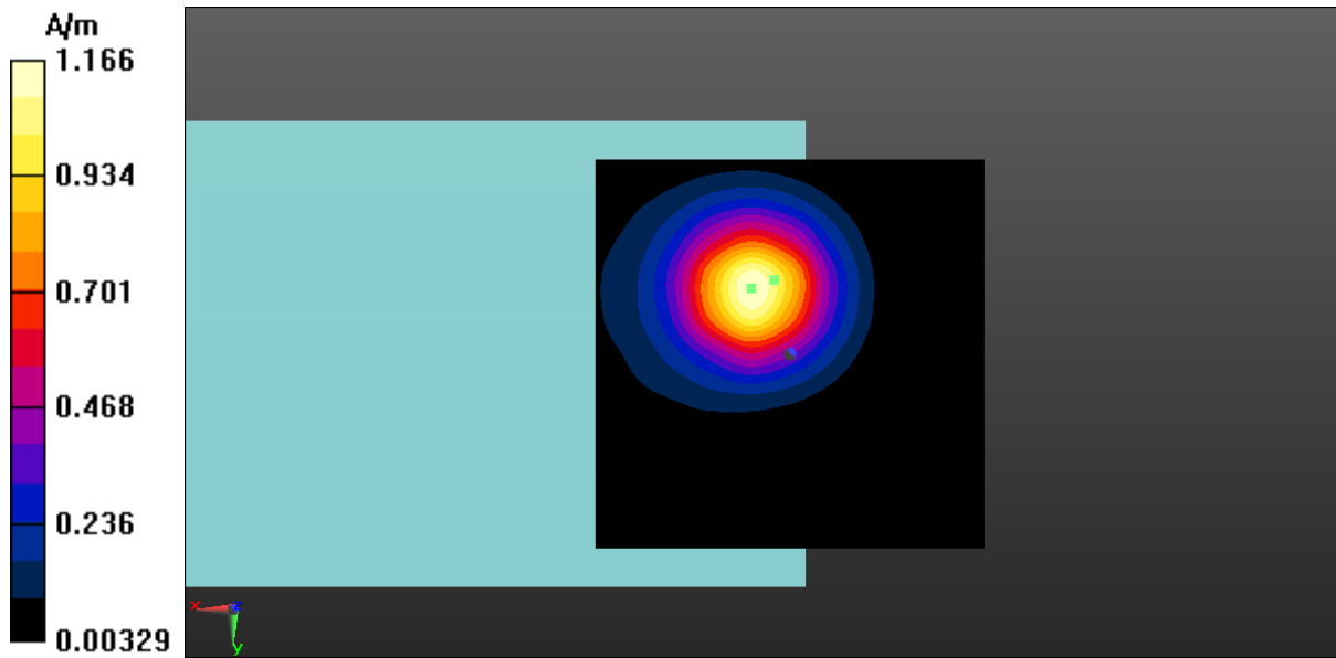
Fig A.14 T-Coil LTE-Band 41-Z
