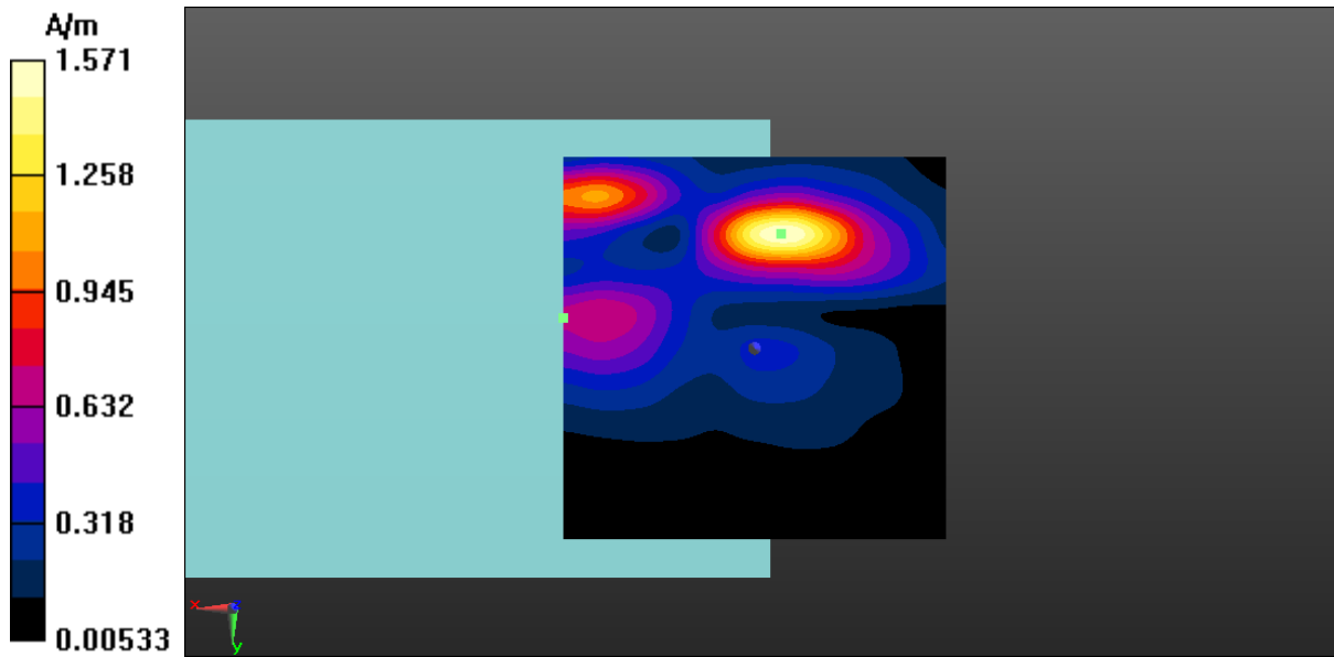
Fig A.2 T-Coil GSM1900-Y
