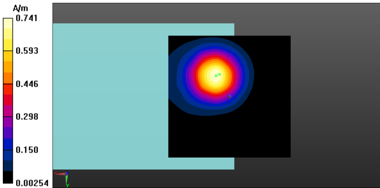
Fig A.15 T-Coil WLAN 2.4GHz-Z
