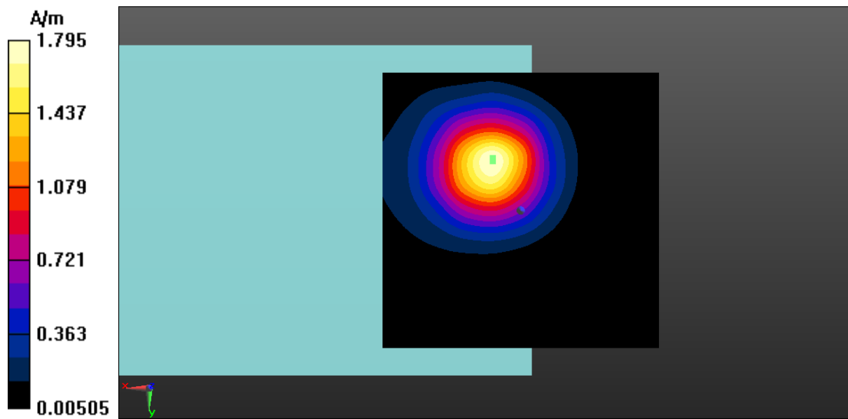
Fig A.21 T-Coil WCDMA Band 4-Z
