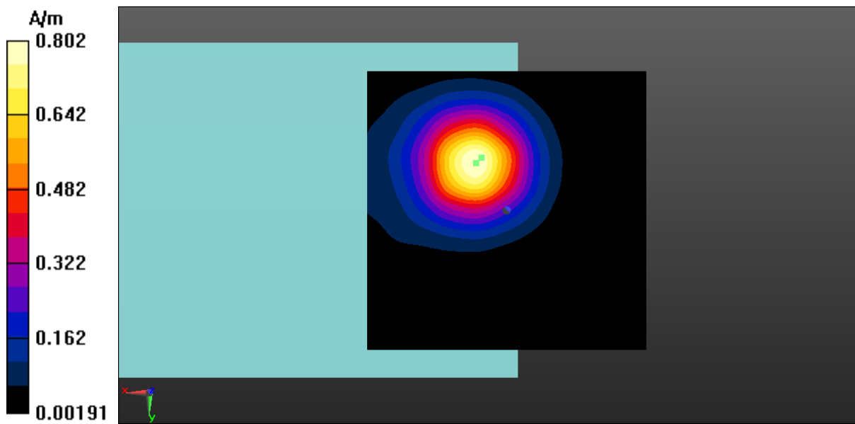
Fig A.17 T-Coil WLAN 5.3GHz-Z
