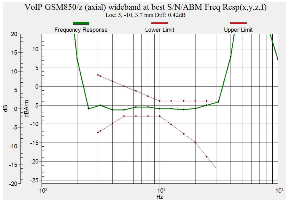
Figure B.20 Frequency Response of GSM 850 (Google Meet)
