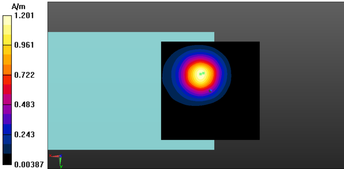
Fig A.10 T-Coil LTE-Band 13-Z
