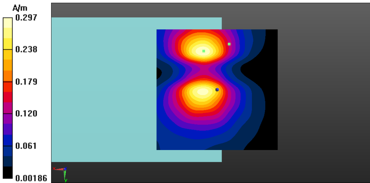
Fig A.15 T-Coil WLAN 2.4GHz-Y
