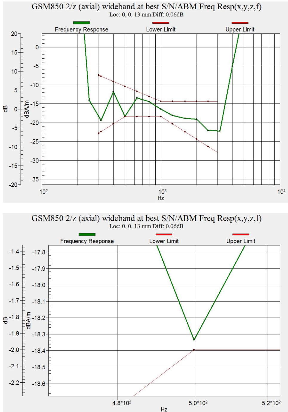
Figure B.1 Frequency Response of GSM850
