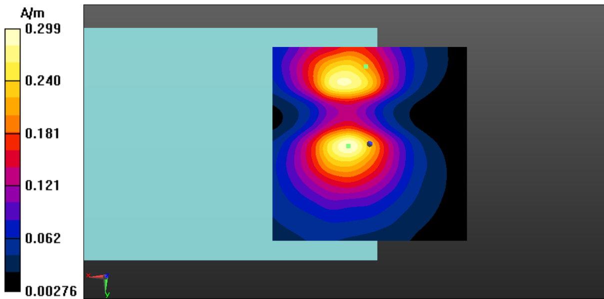
Fig A.16 T-Coil WLAN 5.2GHz-Y
