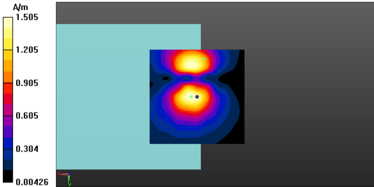
Fig A.13 T-Coil LTE-Band 71-Y
