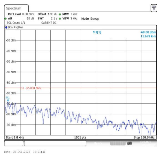
Band41_5MHz_16QAM_40620_1RB#0_0.009~0.15 5_0.009~0.15
