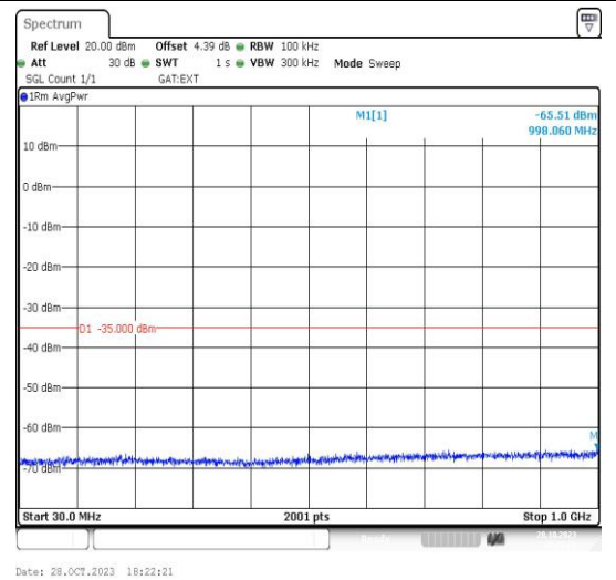
Band41_5MHz_16QAM_40620_1RB#0_30~1000_ 30~1000
