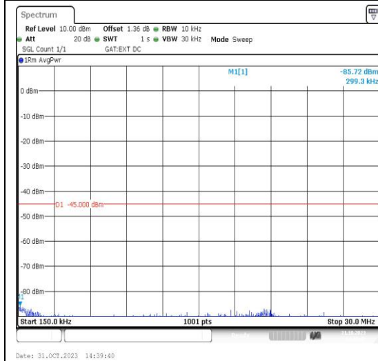
Band41_15MHz_16QAM_39725_1RB#0_0.15~30_0.15~30
