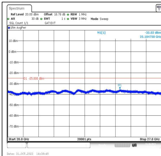
Band41_15MHz_QPSK_39725_1RB#0_20000~27000_20000~27000
