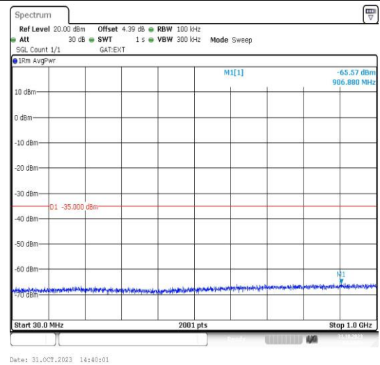
Band41_15MHz_16QAM_39725_1RB#0_30~1000_30~1000
