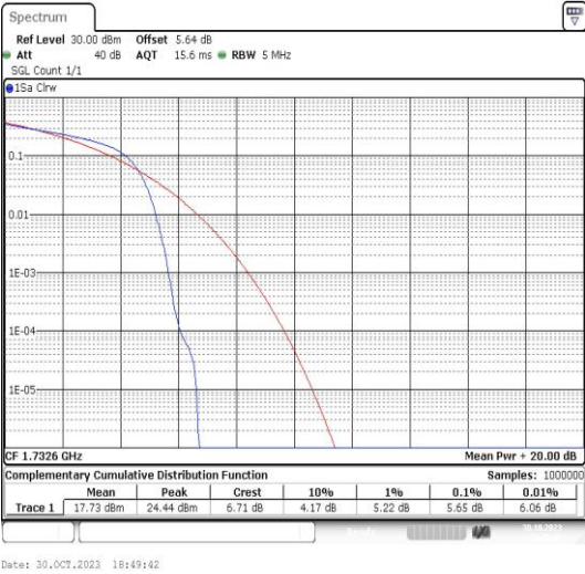
Band4-1413-2-PASS
