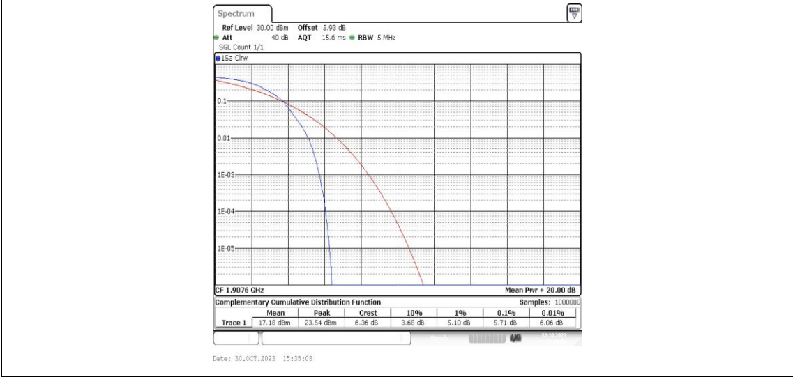
Band2-9538-4-PASS
