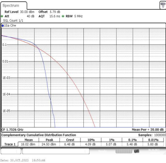
Band4-1513-2-PASS
