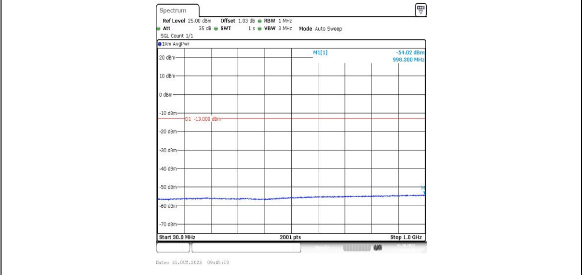
Band4-1513-1-30~1000MHz-PASS
