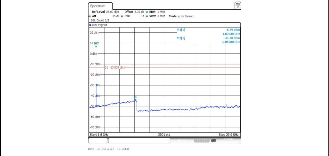
Band2-9400-2-1000~20000MHz-PASS
