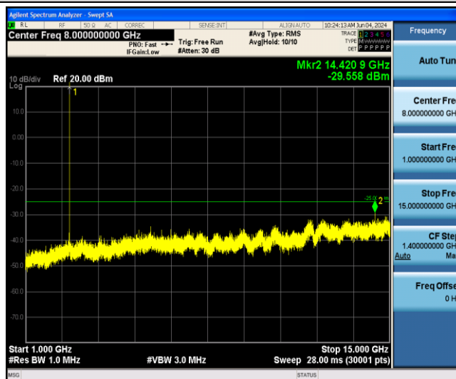
Band41-5MHz-QPSK-41565-1RB#0-Range2:1000~15000MHz
