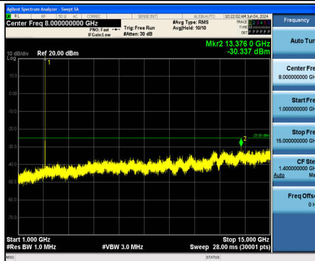
Band41-5MHz-16QAM-39675-1RB#0-Range2:1000~15000MHz
