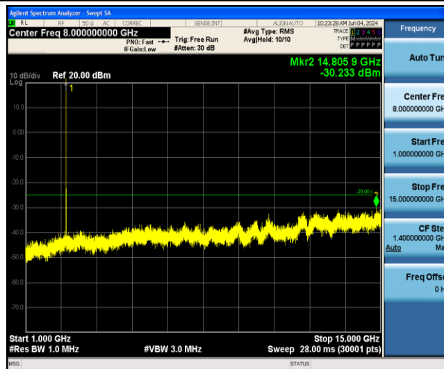
Band41-5MHz-16QAM-40620-1RB#0-Range2:1000~15000MHz
