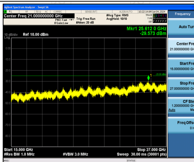
Band41-5MHz-16QAM-39675-1RB#0-Range3:15000~27000MHz
