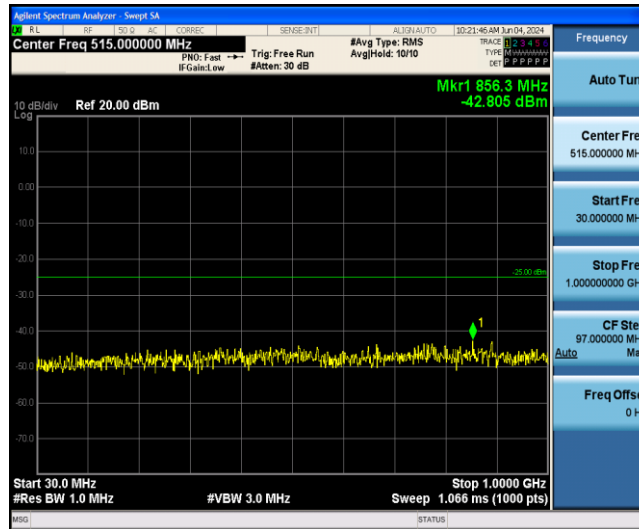
Band41-5MHz-16QAM-39675-1RB#0-Range1:30~1000MHz
