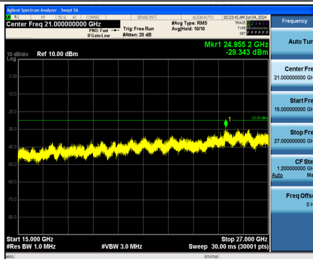
Band41-5MHz-16QAM-40620-1RB#0-Range3:15000~27000MHz
