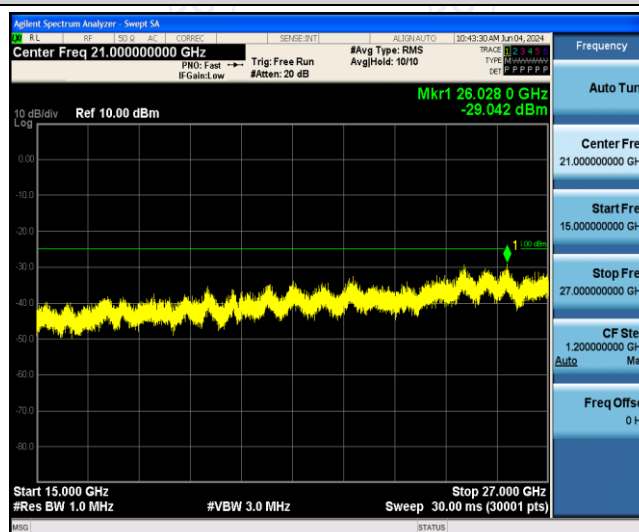
Band41-15MHz-QPSK-39725-1RB#0-Range3:15000~27000MHz
