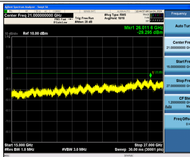
Band41-15MHz-QPSK-40620-1RB#0-Range3:15000~27000MHz
