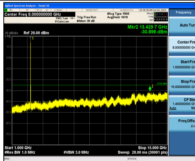
Band41-10MHz-QPSK-41540-1RB#0-Range2:1000~15000MHz
