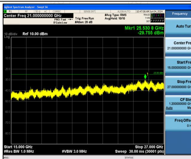
Band41-15MHz-16QAM-41515-1RB#0-Range3:15000~27000MHz
