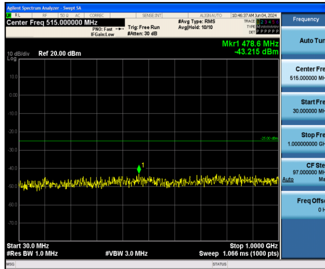
Band41-15MHz-16QAM-41515-1RB#0-Range1:30~1000MHz
