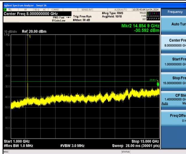
Band41-10MHz-16QAM-40620-1RB#0-Range2:1000~15000MHz
