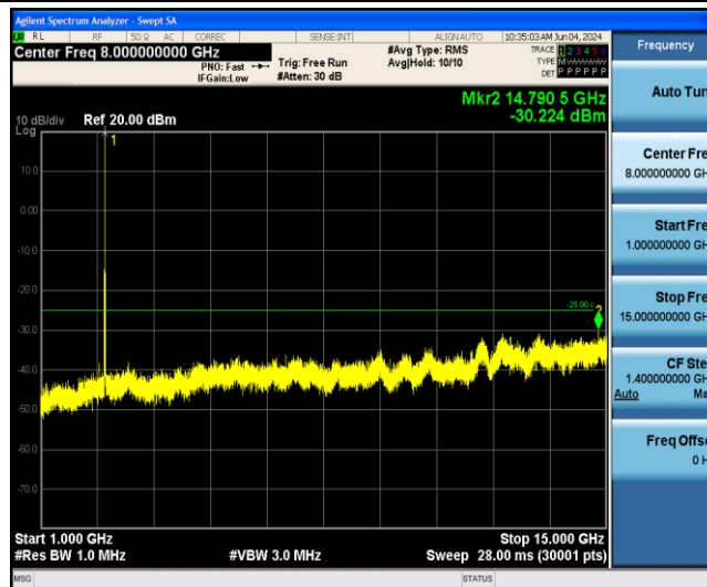
Band41-10MHz-QPSK-40620-1RB#0-Range2:1000~15000MHz
