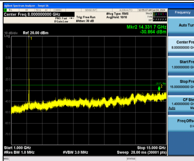
Band41-20MHz-16QAM-40620-1RB#0-Range2:1000~15000MHz
