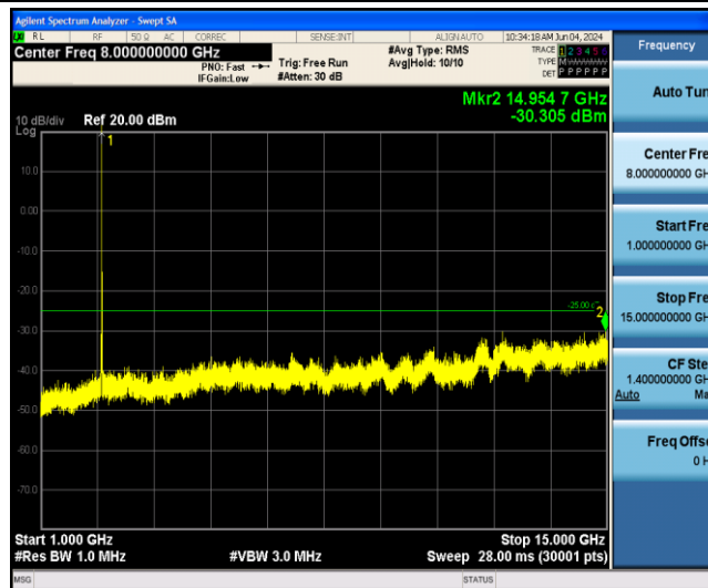
Band41-10MHz-16QAM-39700-1RB#0-Range2:1000~15000MHz
