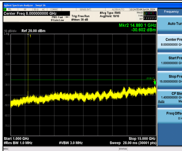
Band41-5MHz-16QAM-41565-1RB#0-Range2:1000~15000MHz
