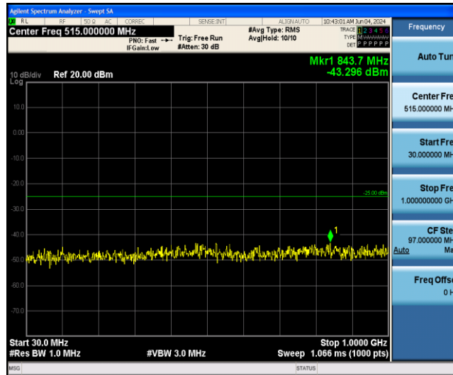
Band41-15MHz-QPSK-39725-1RB#0-Range1:30~1000MHz
