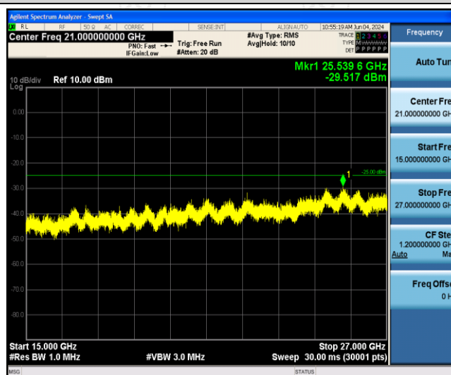
Band41-20MHz-16QAM-40620-1RB#0-Range3:15000~27000MHz
