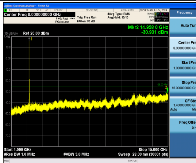
Band41-20MHz-QPSK-40620-1RB#0-Range2:1000~15000MHz
