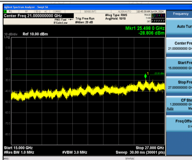
Band41-15MHz-16QAM-40620-1RB#0-Range3:15000~27000MHz
