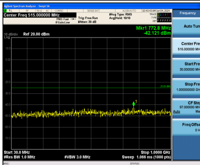
Band41-15MHz-16QAM-39725-1RB#0-Range1:30~1000MHz
