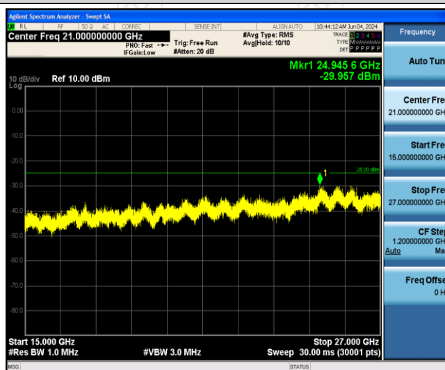
Band41-15MHz-16QAM-39725-1RB#0-Range3:15000~27000MHz
