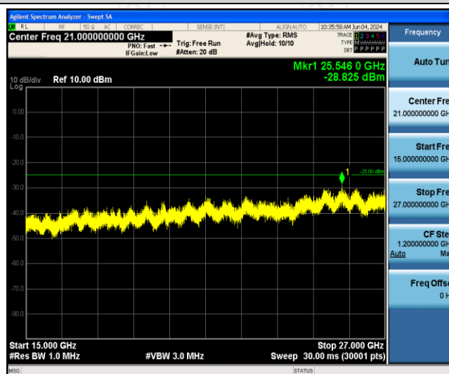
Band41-10MHz-16QAM-40620-1RB#0-Range3:15000~27000MHz
