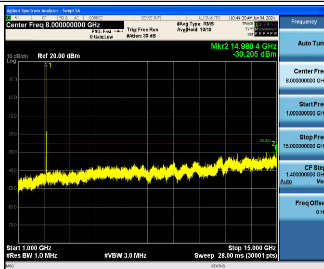
Band41-15MHz-16QAM-39725-1RB#0-Range2:1000~15000MHz
