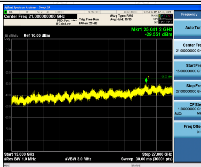
Band41-20MHz-QPSK-40620-1RB#0-Range3:15000~27000MHz
