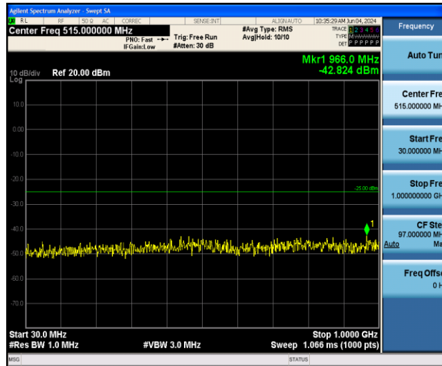
Band41-10MHz-16QAM-40620-1RB#0-Range1:30~1000MHz
