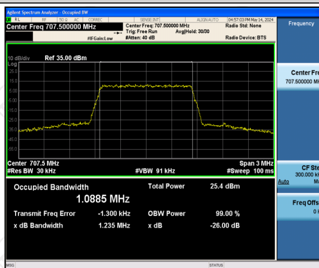
Band12-1.4MHz-16QAM-23095-6RB#0
