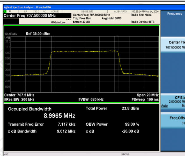
Band12-10MHz-16QAM-23095-50RB#0
