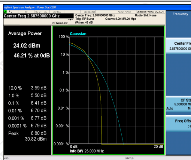
Band41-5MHz-16QAM-41565-1RB#0
