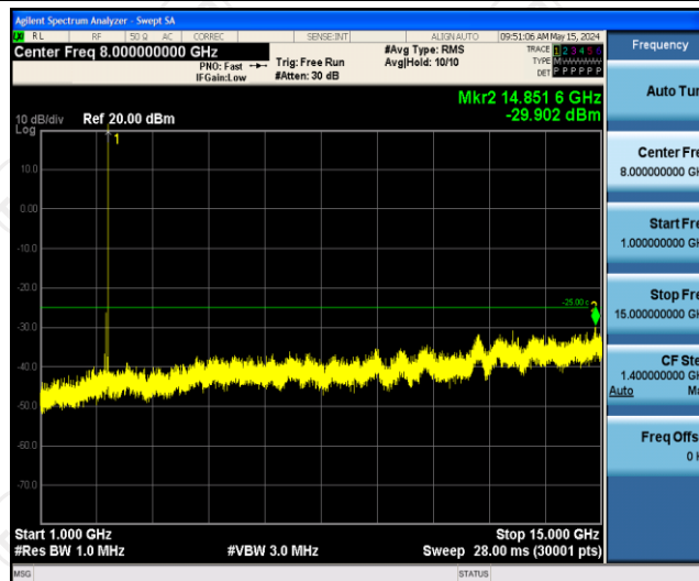
Band41-5MHz-QPSK-41565-1RB#0-Range2:1000~15000MHz
