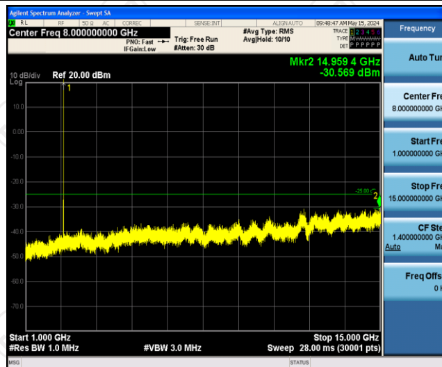
Band41-5MHz-16QAM-39675-1RB#0-Range2:1000~15000MHz
