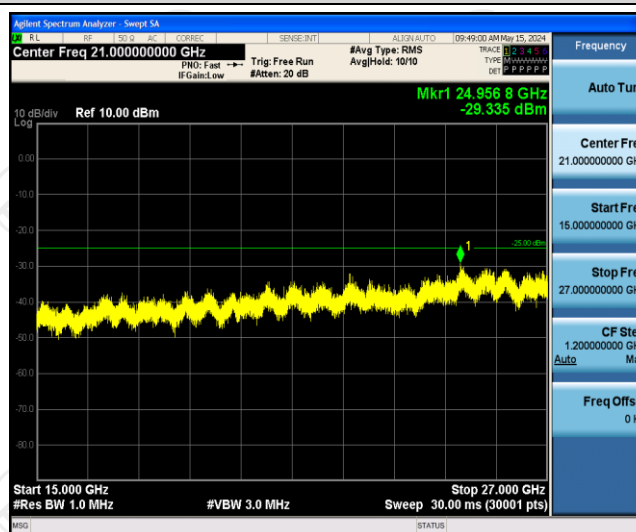
Band41-5MHz-16QAM-39675-1RB#0-Range3:15000~27000MHz
