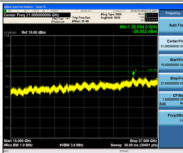
Band41-5MHz-16QAM-40620-1RB#0-Range3:15000~27000MHz
