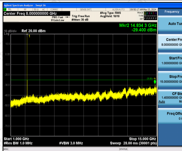
Band41-5MHz-16QAM-40620-1RB#0-Range2:1000~15000MHz
