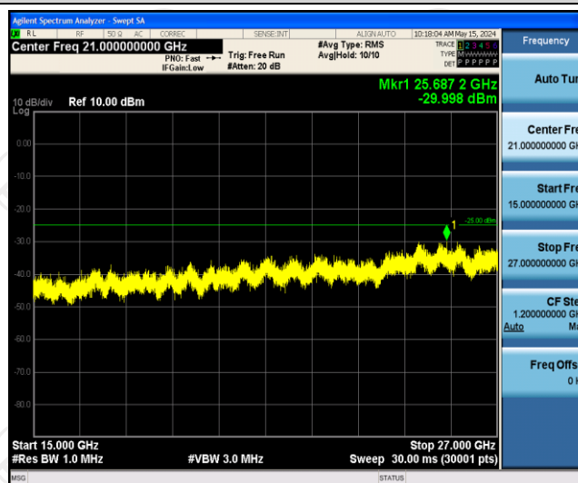
Band41-20MHz-16QAM-39750-1RB#0-Range3:15000~27000MHz
