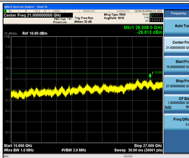
Band41-10MHz-16QAM-41540-1RB#0-Range3:15000~27000MHz
