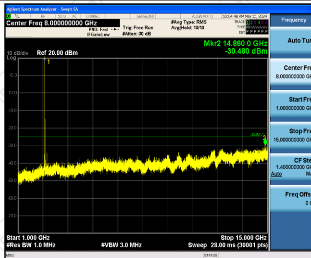
Band41-15MHz-QPSK-39725-1RB#0-Range2:1000~15000MHz
