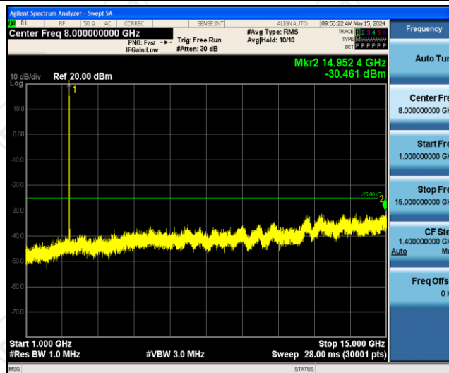
Band41-10MHz-16QAM-41540-1RB#0-Range2:1000~15000MHz
