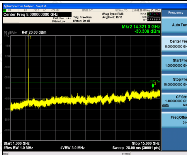
Band41-15MHz-16QAM-41515-1RB#0-Range2:1000~15000MHz
