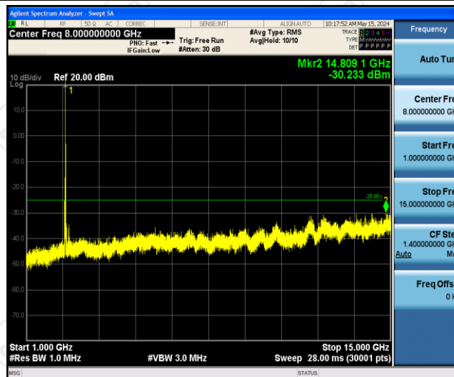
Band41-20MHz-16QAM-39750-1RB#0-Range2:1000~15000MHz
