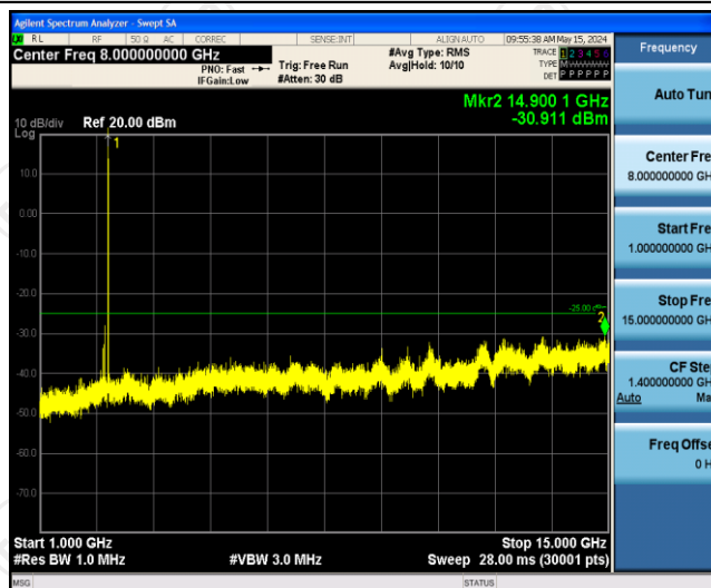
Band41-10MHz-QPSK-41540-1RB#0-Range2:1000~15000MHz
