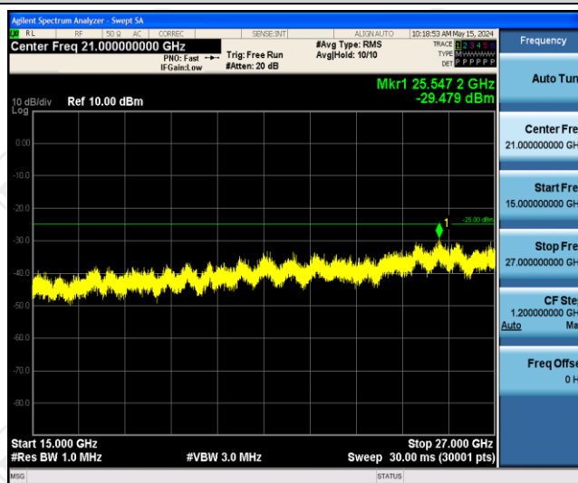
Band41-20MHz-QPSK-40620-1RB#0-Range3:15000~27000MHz
