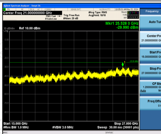
Band41-15MHz-QPSK-39725-1RB#0-Range3:15000~27000MHz
