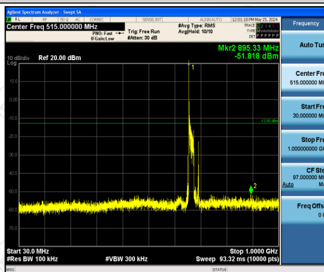
Band71-20MHz-16QAM-133222-1RB#0-Range1:30~1000MHz
