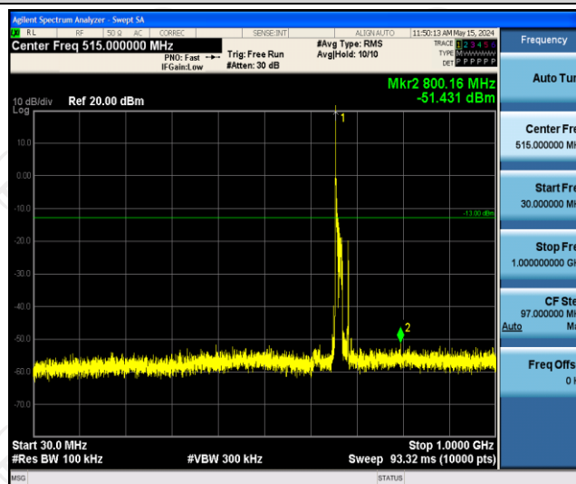
Band71-15MHz-QPSK-133197-1RB#0-Range1:30~1000MHz
