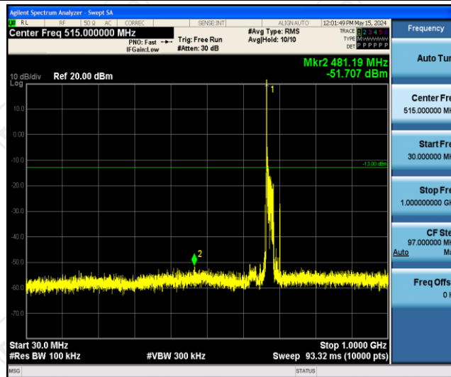
Band71-20MHz-QPSK-133322-1RB#0-Range1:30~1000MHz
