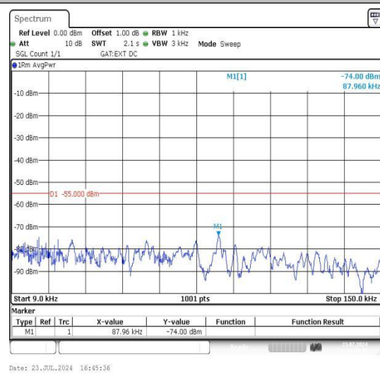
Band41_20MHz_QPSK_40620_1RB#0_0.009~0.15 15_0.009~0.15
