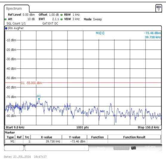
Band41_20MHz_16QAM_40620_1RB#0_0.009~0.15_0.009~0.15
