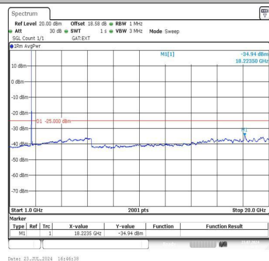
Band41_20MHz_QPSK_40620_1RB#0_1000~20000 00_1000~20000
