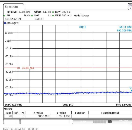
Band41_20MHz_QPSK_40620_1RB#0_30~1000 _30~1000
