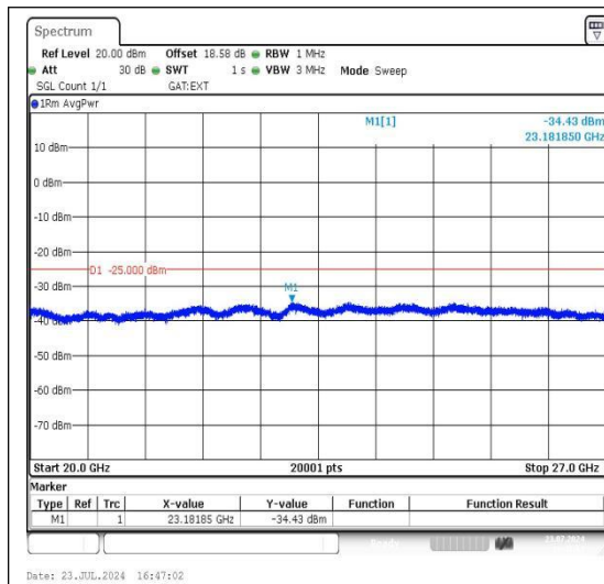
Band41_20MHz_QPSK_40620_1RB#0_20000~27000_20000~27000
