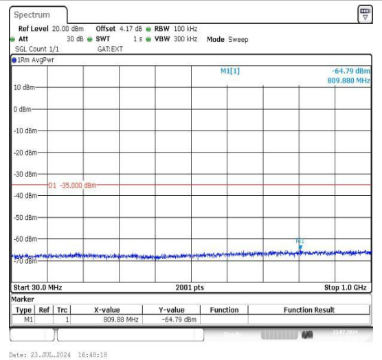
Band41_20MHz_16QAM_40620_1RB#0_30~1000_30~1000
