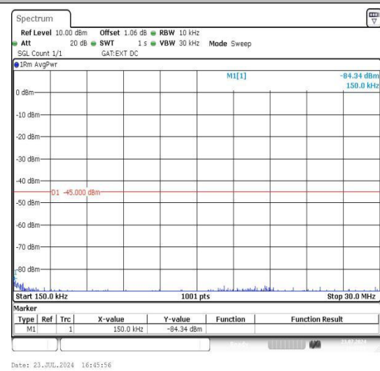
Band41_20MHz_QPSK_40620_1RB#0_0.15~30 0.15~30
