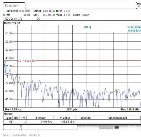
Band66_10MHz_16QAM_132322_1RB#0_0.009~ 0.15_0.009~0.15
