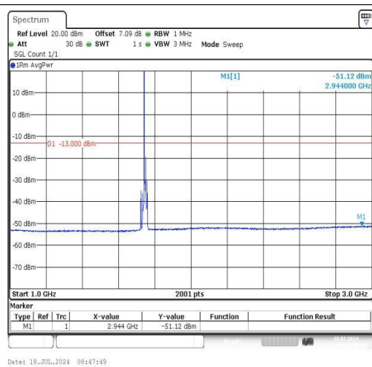
Band66_10MHz_QPSK_132322_1RB#0_1000~30 00_1000~3000
