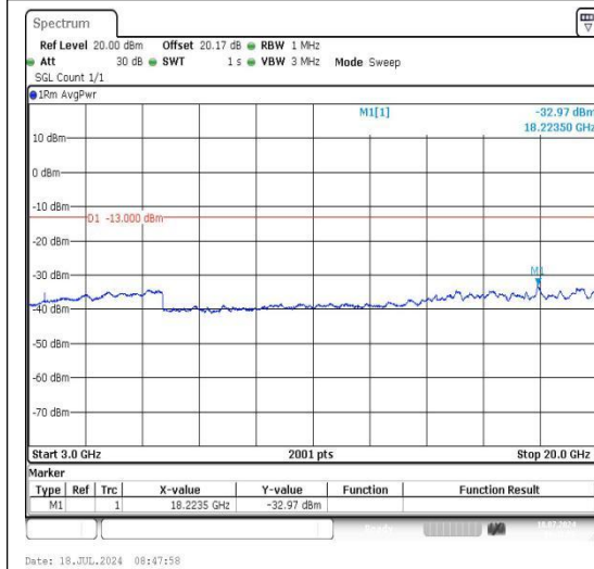
Band66_10MHz_QPSK_132322_1RB#0_3000~2 0000_3000~20000
