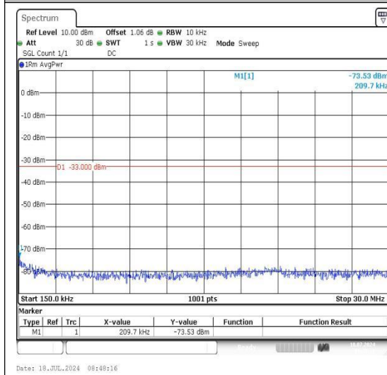
Band66_10MHz_QPSK_132322_1RB#0_3000~2 0000_3000~20000
