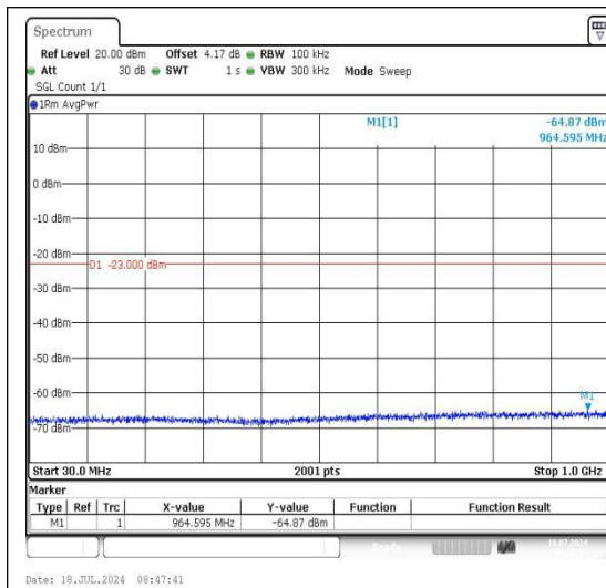
Band66_10MHz_QPSK_132322_1RB#0_30~100 0_30~1000
