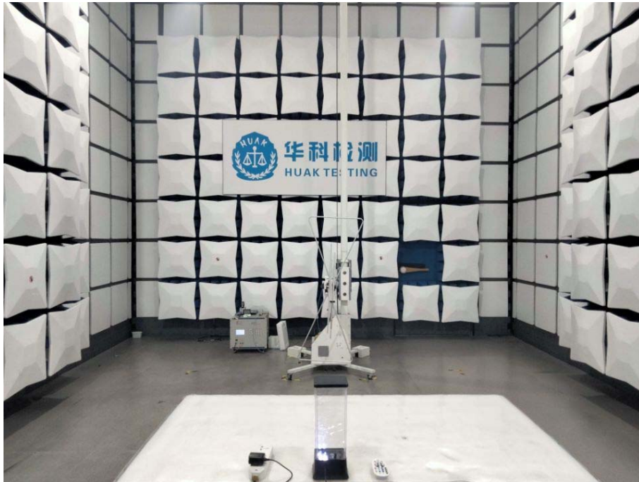
Model: BH-BTJ01 Radiated Emissions
