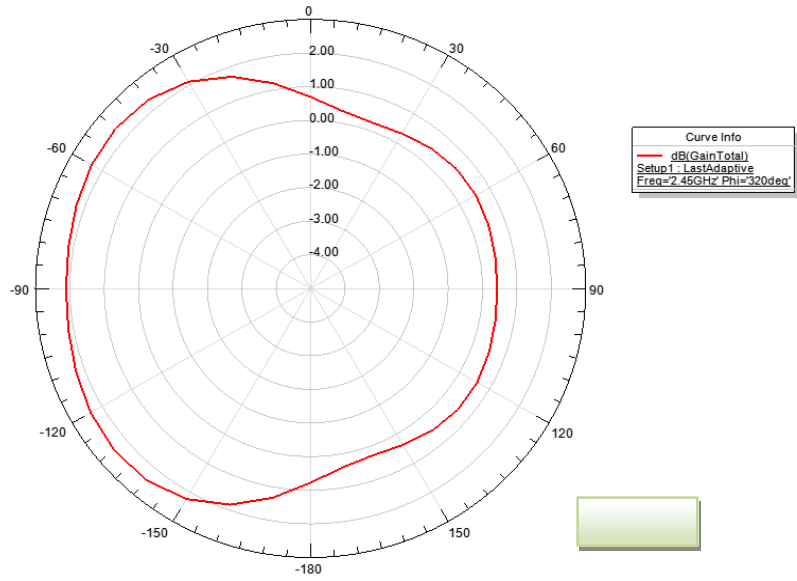
E plan
