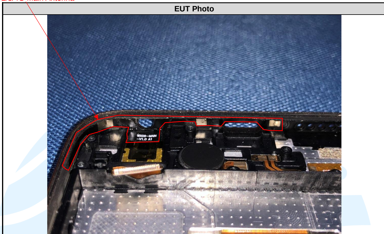
2/3/4G Main Antenna
