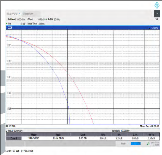
Band2-20MHz-64QAM-19100-100RB#0-PASS
