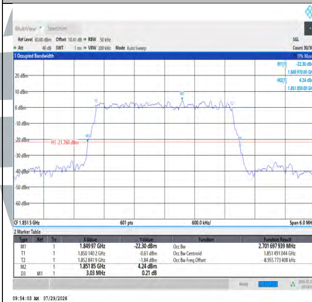
Band2-3MHz-16QAM-18615-15RB#0-PASS
