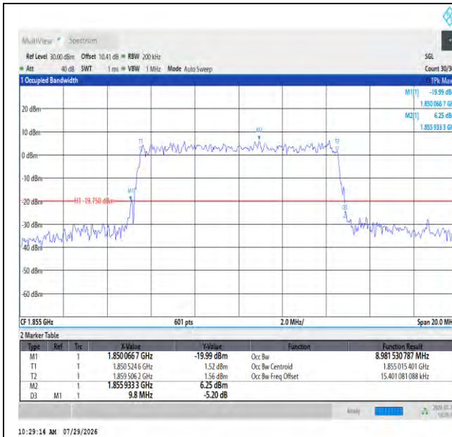
Band2-10MHz-16QAM-18650-50RB#0-PASS
