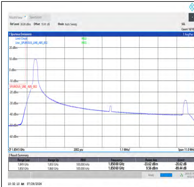
Band2-10MHz-64QAM-18650-1RB#0-PASS
