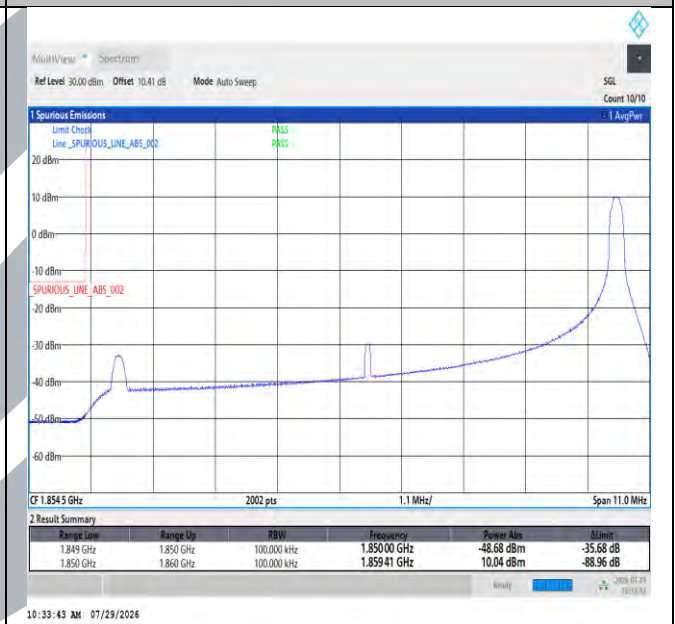
Band2-10MHz-64QAM-18650-1RB#49-PASS
