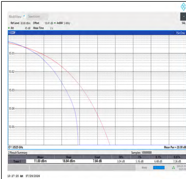
Band2-5MHz-64QAM-18625-25RB#0-PASS
