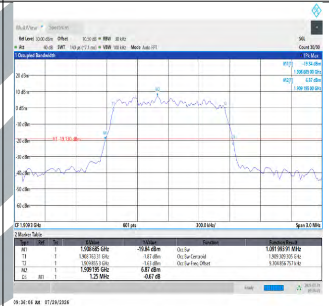
Band2-1.4MHz-16QAM-19193-6RB#0-PASS
