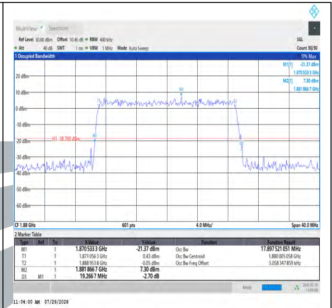
Band2-20MHz-16QAM-18900-100RB#0-PASS
