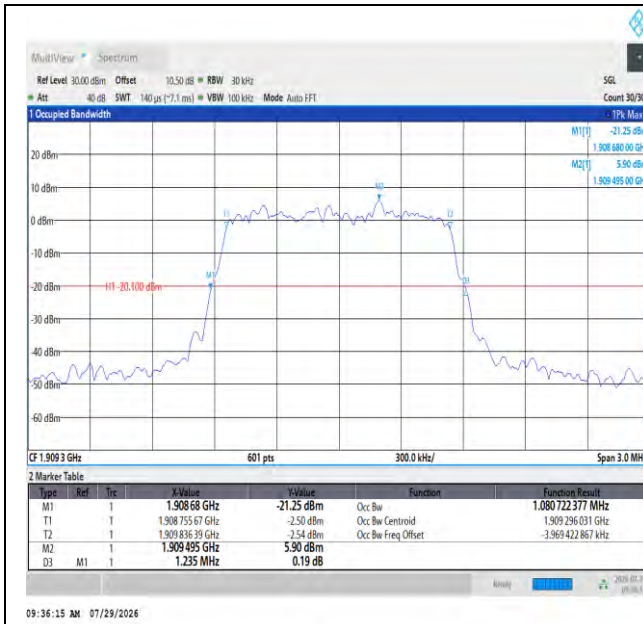
Band2-1.4MHz-64QAM-19193-6RB#0-PASS
