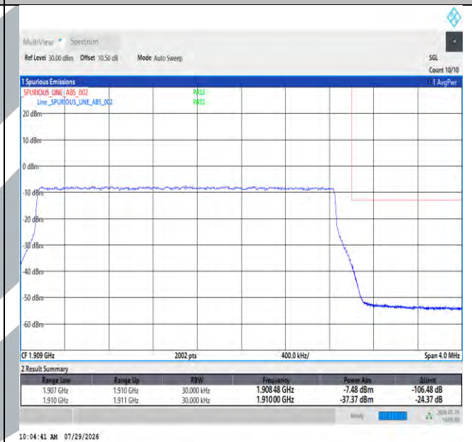
Band2-3MHz-64QAM-19185-15RB#0-PASS
