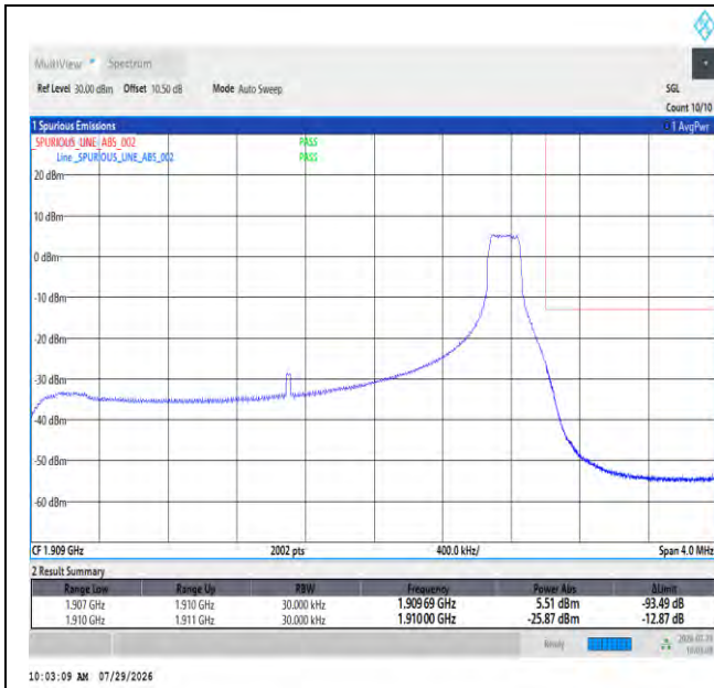
Band2-3MHz-64QAM-19185-1RB#14-PASS
