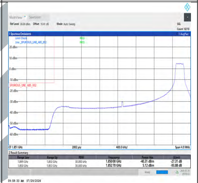
Band2-3MHz-64QAM-18615-1RB#14-PASS
