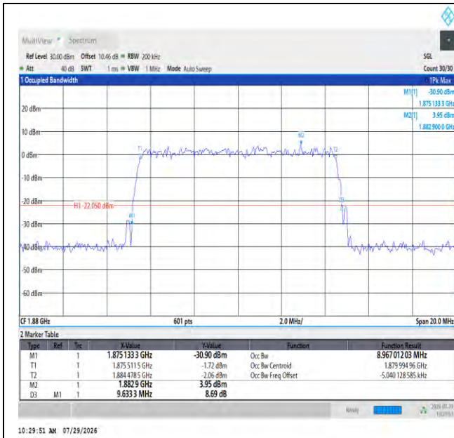
Band2-10MHz-64QAM-18900-50RB#0-PASS
