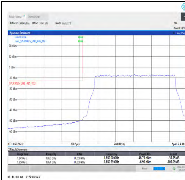
Band2-1.4MHz-64QAM-18607-6RB#0-PASS
