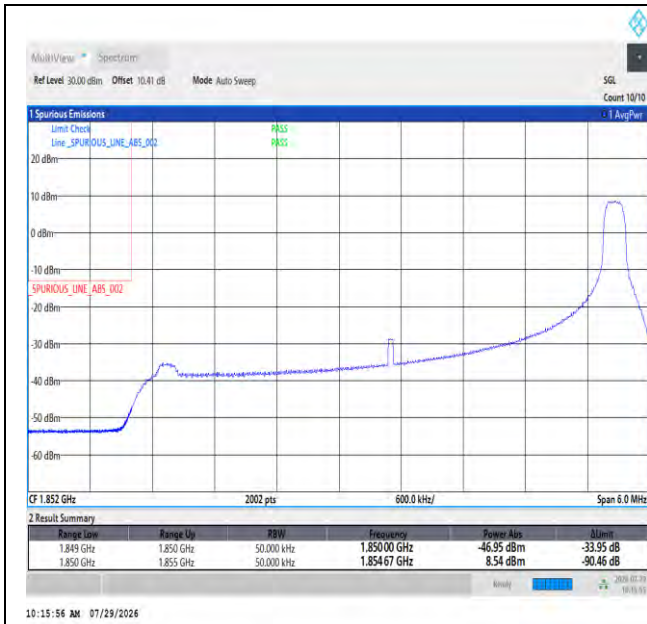
Band2-5MHz-16QAM-18625-1RB#24-PASS
