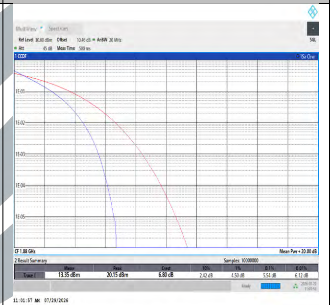
Band2-15MHz-QPSK-18900-75RB#0-PASS
