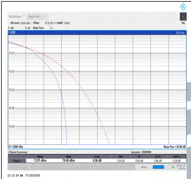
Band2-3MHz-16QAM-19185-15RB#0-PASS
