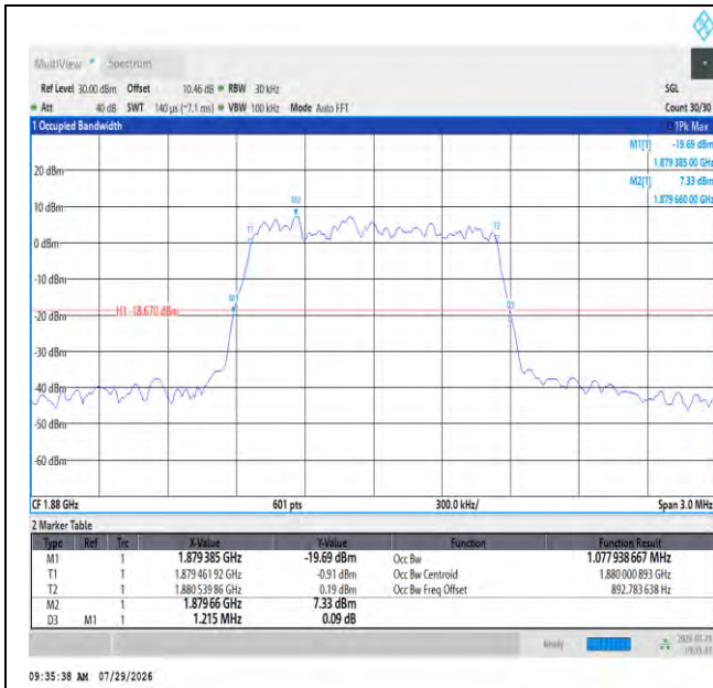
Band2-1.4MHz-16QAM-18900-6RB#0-PASS
