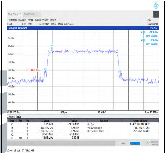
Band2-15MHz-16QAM-18675-75RB#0-PASS
