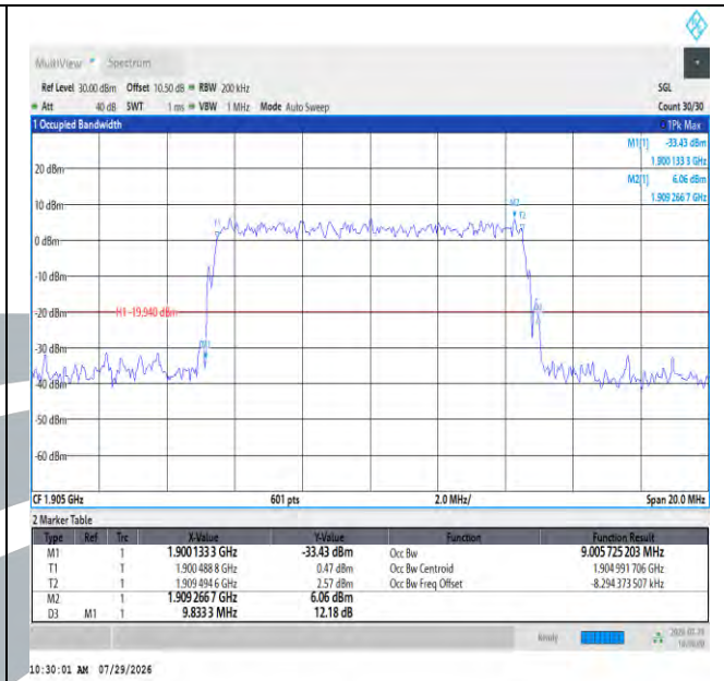
Band2-10MHz-QPSK-19150-50RB#0-PASS
