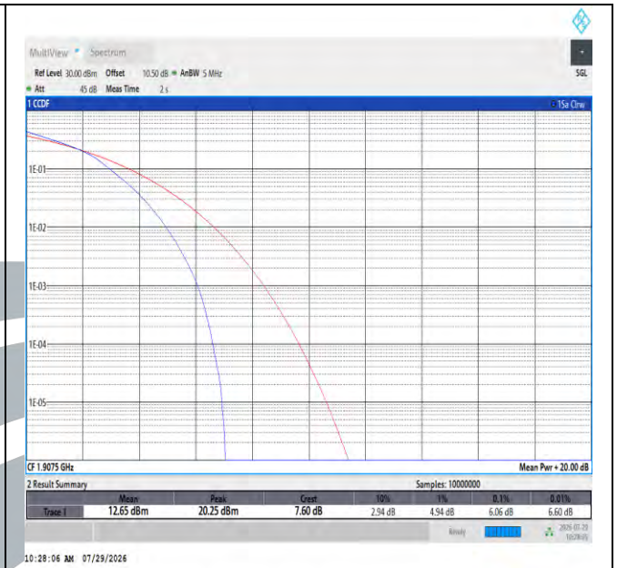
Band2-5MHz-16QAM-19175-25RB#0-PASS
