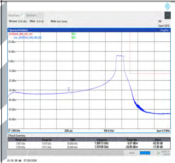
Band2-3MHz-16QAM-19185-1RB#14-PASS
