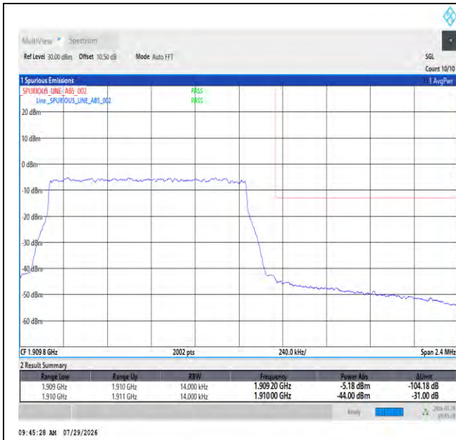
Band2-1.4MHz-16QAM-19193-6RB#0-PASS
