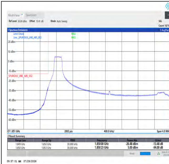
Band2-3MHz-64QAM-18615-1RB#0-PASS
