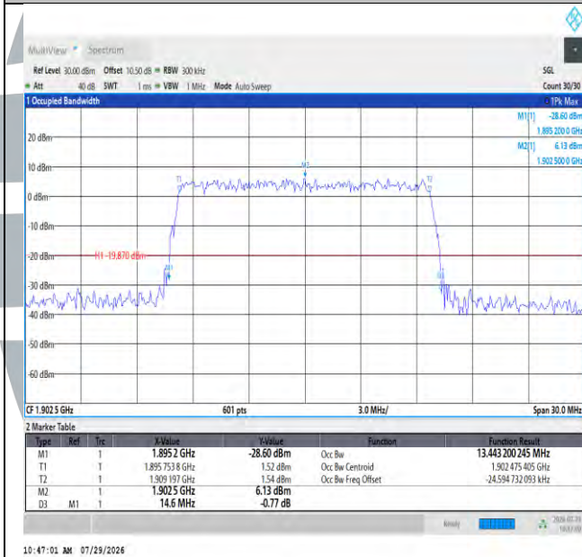
Band2-15MHz-QPSK-19125-75RB#0-PASS
