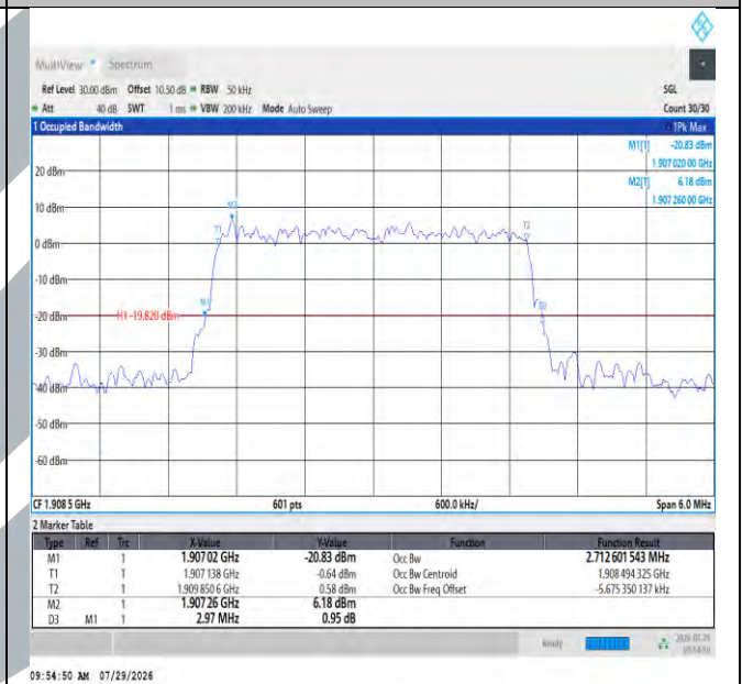
Band2-3MHz-QPSK-19185-15RB#0-PASS
