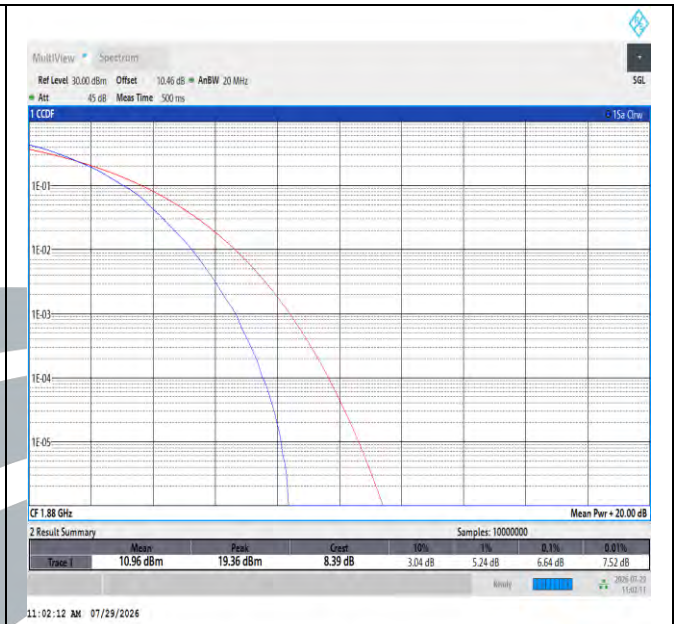
Band2-15MHz-64QAM-18900-75RB#0-PASS
