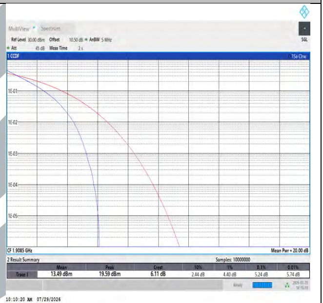
Band2-3MHz-QPSK-19185-15RB#0-PASS
