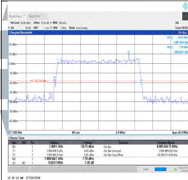
Band2-10MHz-16QAM-19150-50RB#0-PASS
