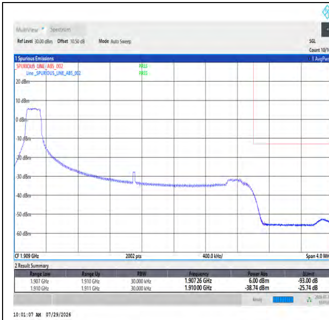
Band2-3MHz-16QAM-19185-1RB#0-PASS
