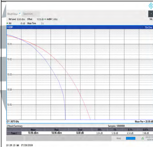
Band2-5MHz-64QAM-19175-25RB#0-PASS
