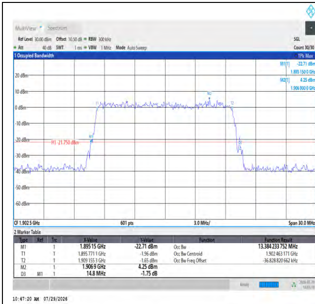
Band2-15MHz-64QAM-19125-75RB#0-PASS
