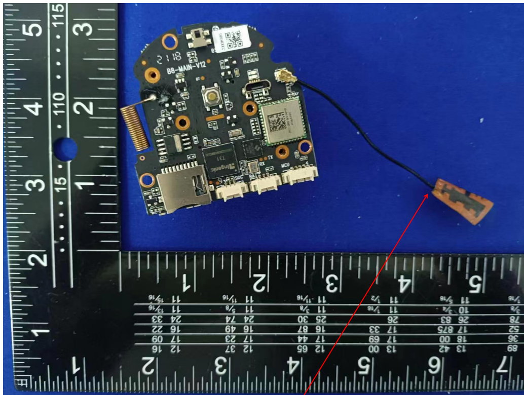
Internal antenna
