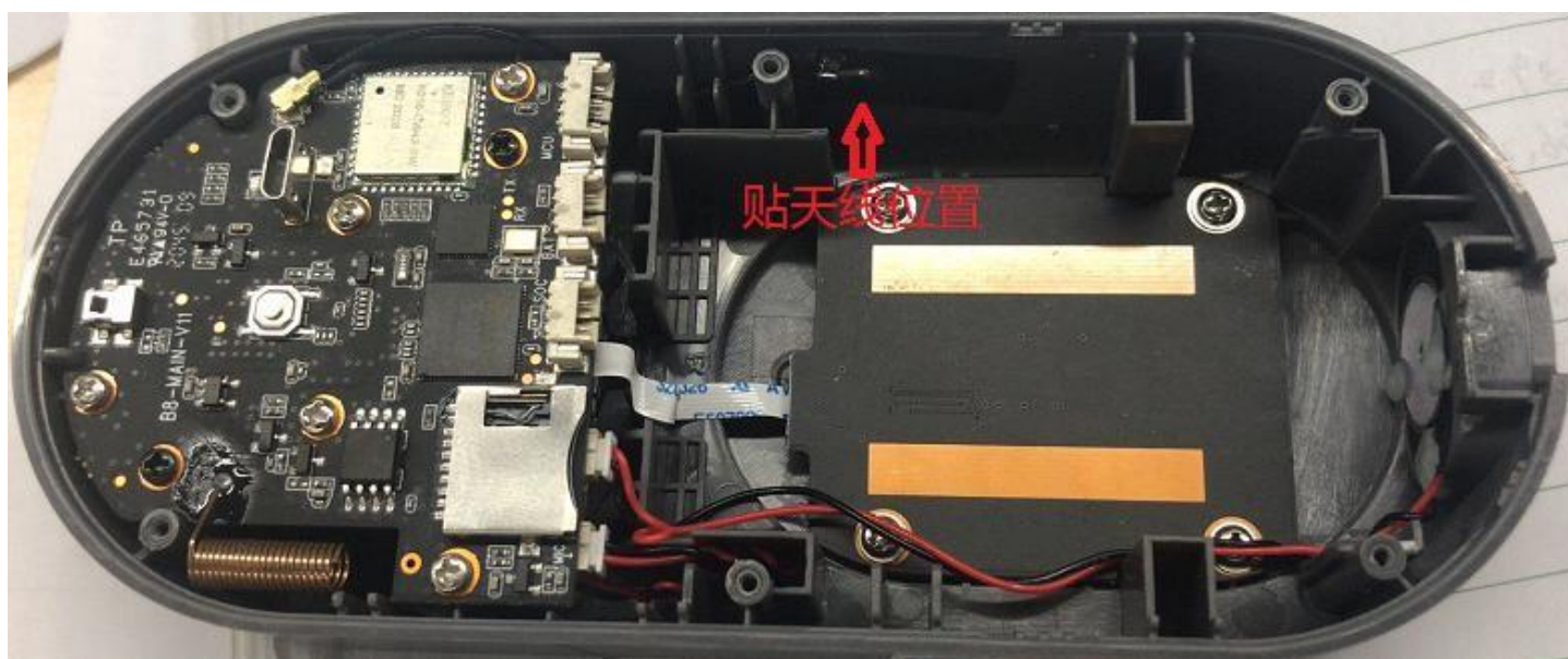
Chart 3 Location of antenna patch
