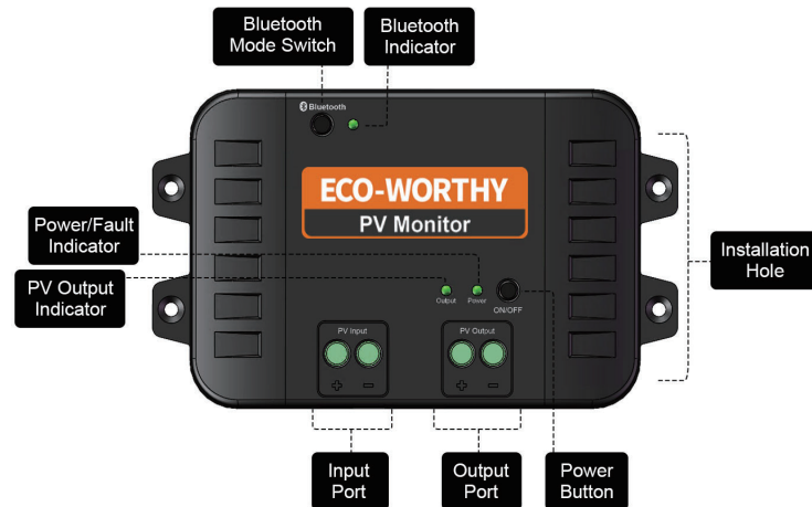
Product Function Indication Diagram
