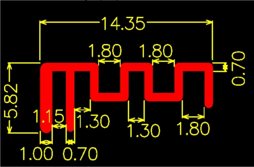
Antenna Photo & Length (mm)
