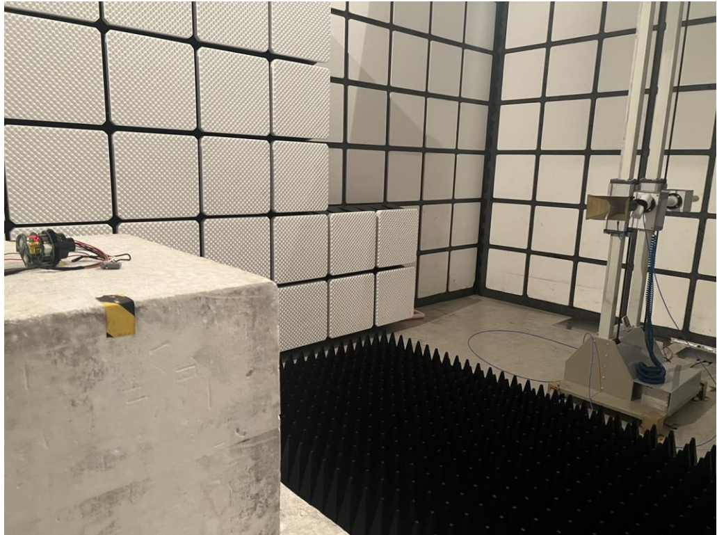
Side View
