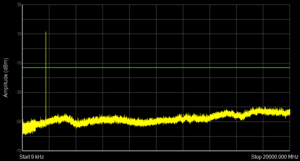
Band66 QPSK BW=10MHz Channel=132622 RB Size=1 Position=#0
