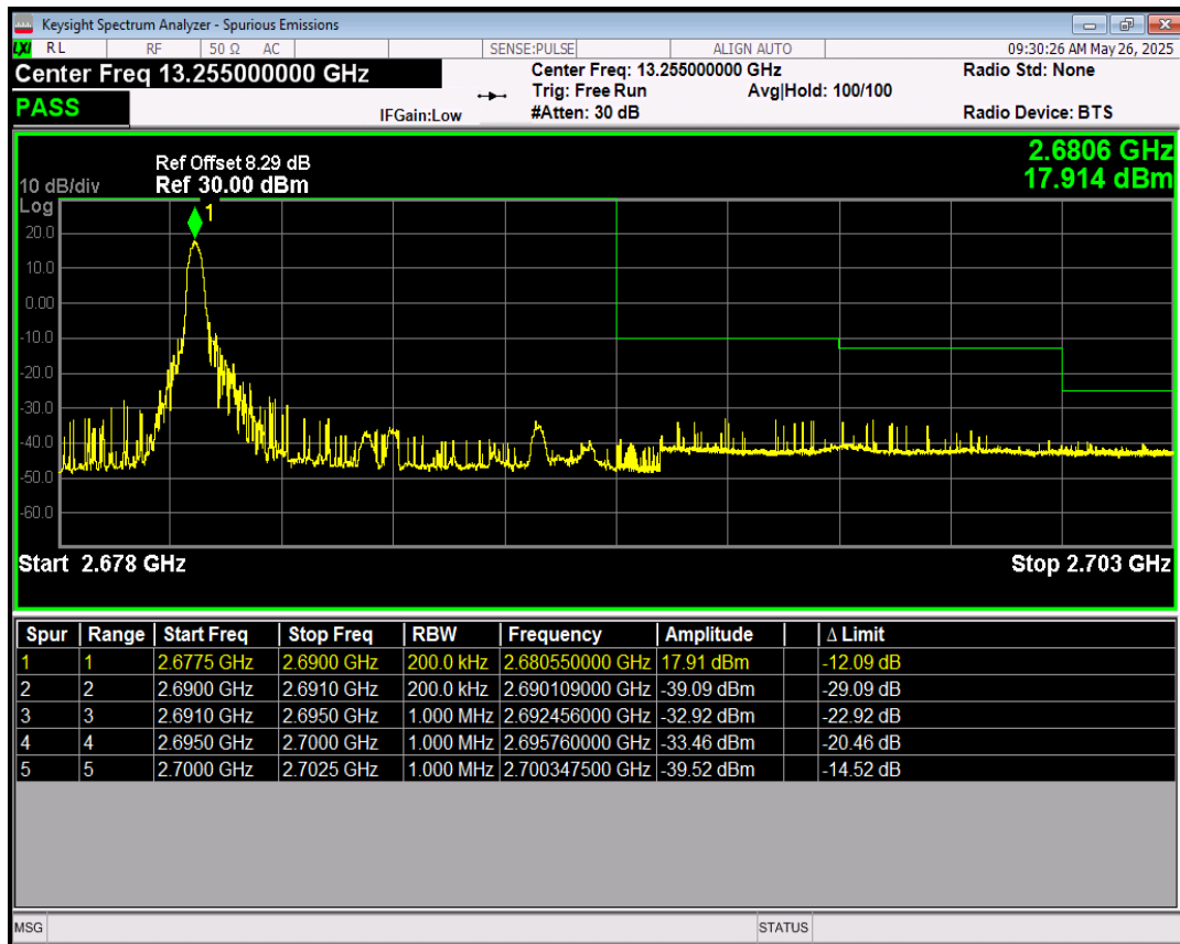
Band41 16QAM BW=10MHz Channel=41540 RB Size=1 Position=#Max
