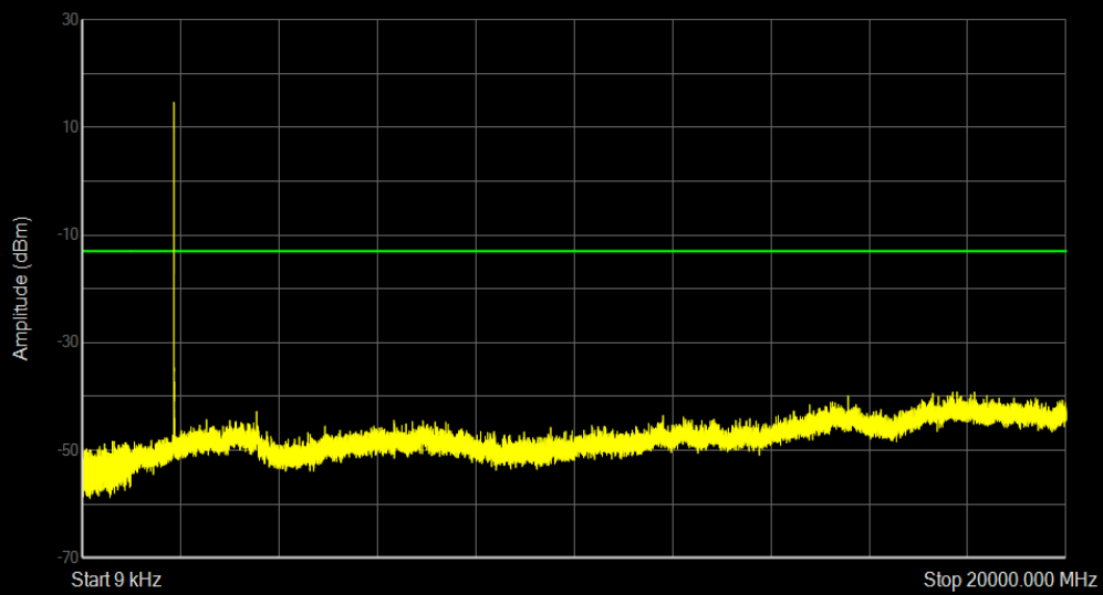
Band25 16QAM BW=10MHz Channel=26365 RB Size=1 Position=#0
