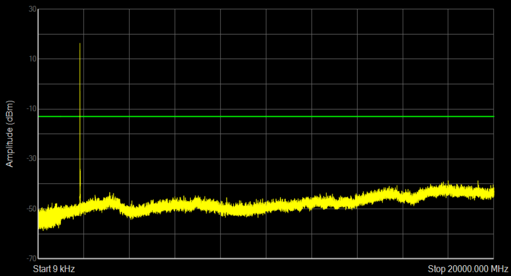
Band25 16QAM BW=15MHz Channel=26115 RB Size=1 Position=#0
