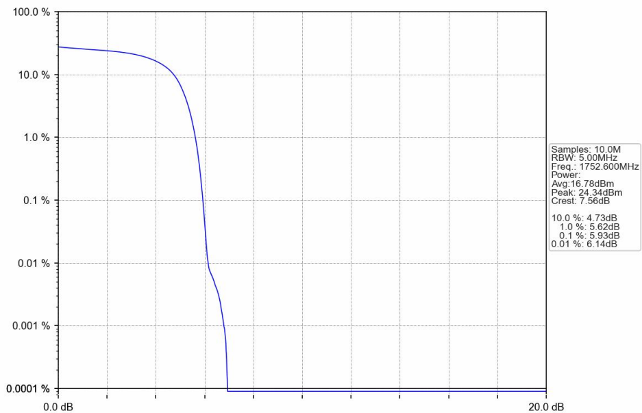
Band4_HSUPA_HCH_1752.6MHz_Subtest 1_NTNV
