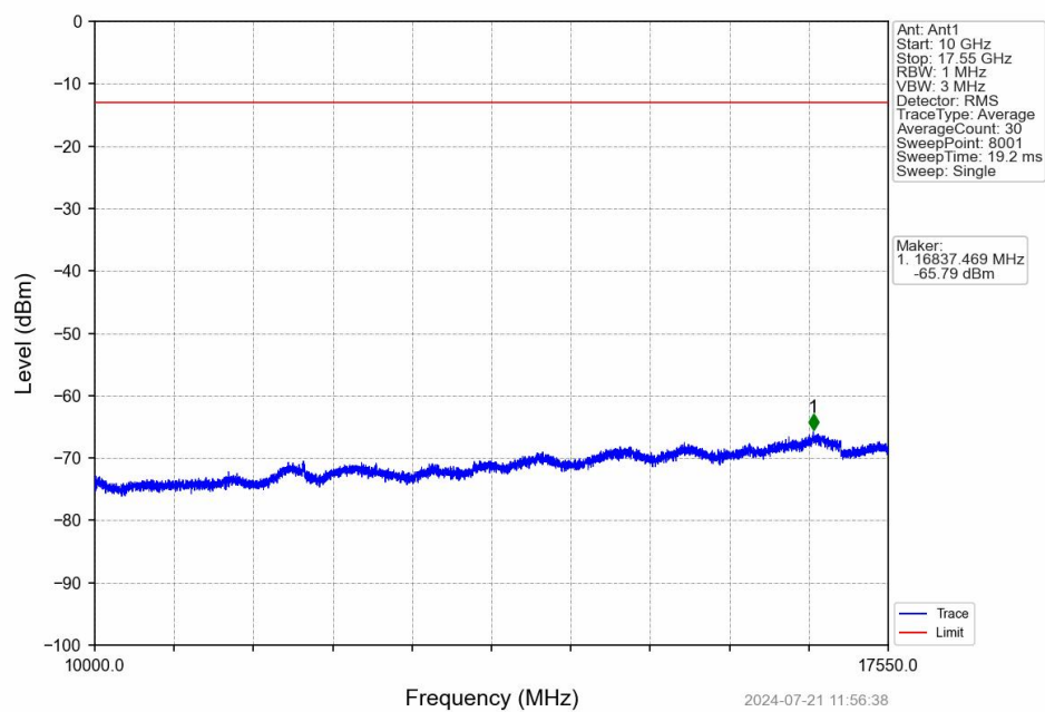
Band4_HSDPA_LCH_1712.4MHz_Subtest 1_NTNV
