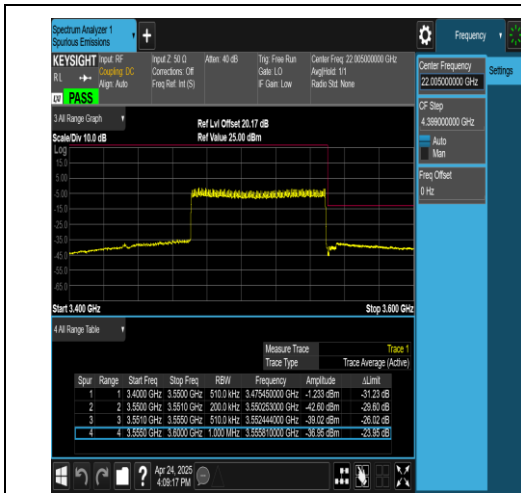
NTNV-N78-3450-3550-PC2-30-80-H-DFT-QPSK-Outer_Full-Ant1-PASS
