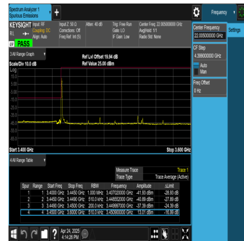
NTNV-N78-3450-3550-PC2-30-90-L-DFT-QPSK-Edge_1RB_Left-Ant1-PASS
