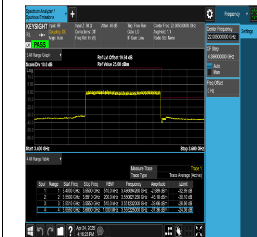
NTNV-N78-3450-3550-PC2-30-90-H-DFT-QPSK-Outer_Full-Ant1-PASS
