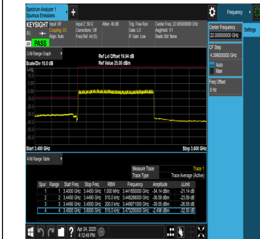
NTNV-N78-3450-3550-PC2-30-90-L-DFT-QPSK-Outer_Full-Ant1-PASS
