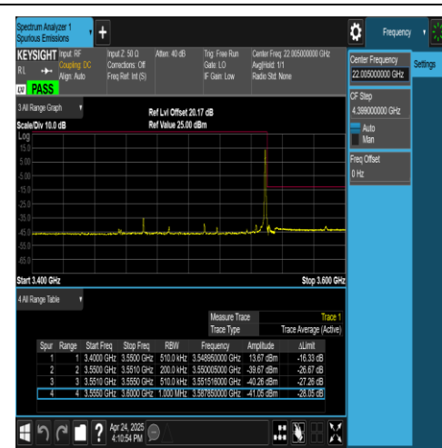
NTNV-N78-3450-3550-PC2-30-80-H-DFT-QPSK-Edge_1RB_Right-Ant1-PASS
