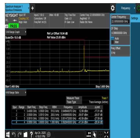
NTNV-N78-3450-3550-PC2-30-90-H-DFT-QPSK-Edge_1RB_Right-Ant1-PASS
