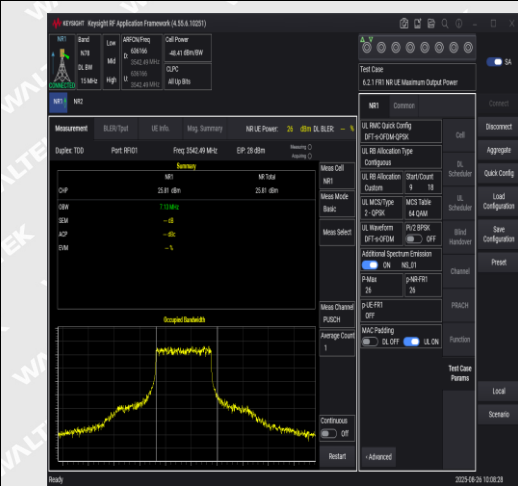
NTNV-N78-3450-3550-PC2-30-15-H-DFT-QPSK-I nner_Full-PASS
