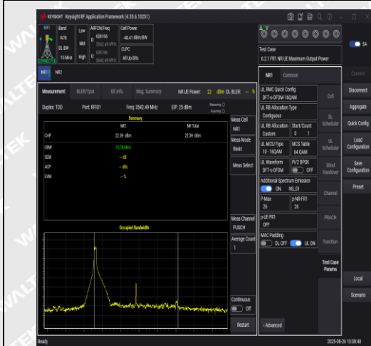
NTNV-N78-3450-3550-PC2-30-15-H-DFT-16QAM- Edge_1RB_Left-PASS
