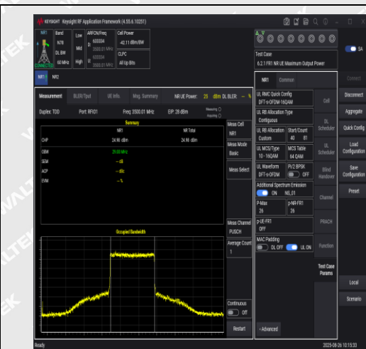
NTNV-N78-3450-3550-PC2-30-60-M-DFT-16QAM -Inner_Full-PASS
