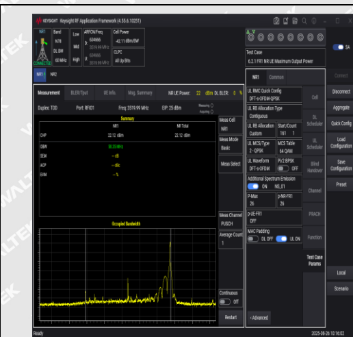
NTNV-N78-3450-3550-PC2-30-60-H-DFT-QPSK- Edge_1RB_Right-PASS
