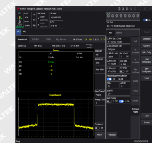
NTNV-N78-3450-3550-PC2-30-60-M-DFT-16QAM -Outer_Full-PASS
