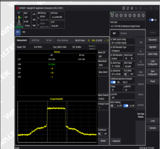
NTNV-N78-3450-3550-PC2-30-70-L-DFT-16QAM- Inner_Full-PASS
