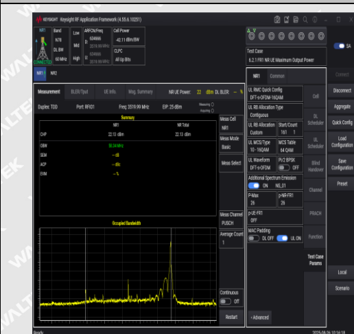
NTNV-N78-3450-3550-PC2-30-60-H-DFT-16QAM- Edge_1RB_Right-PASS
