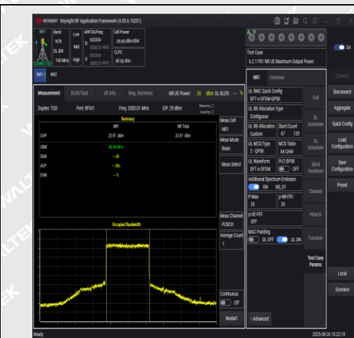
NTNV-N78-3450-3550-PC2-30-100-L-DFT-QPSK- Inner_Full-PASS
