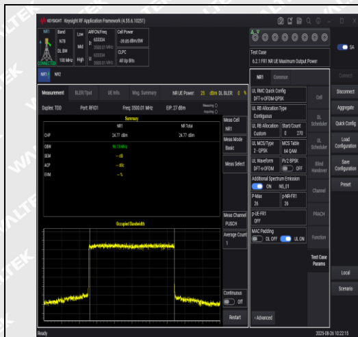
NTNV-N78-3450-3550-PC2-30-100-L-DFT-QPSK- Outer_Full-PASS
