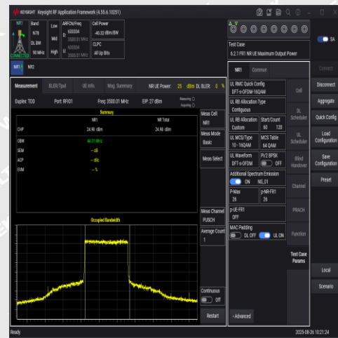
NTNV-N78-3450-3550-PC2-30-90-M-DFT-16QAM -Inner_Full-PASS
