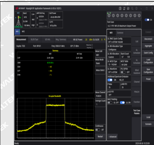
NTNV-N78-3450-3550-PC2-30-100-M-DFT-16QA M-Inner_Full-PASS
