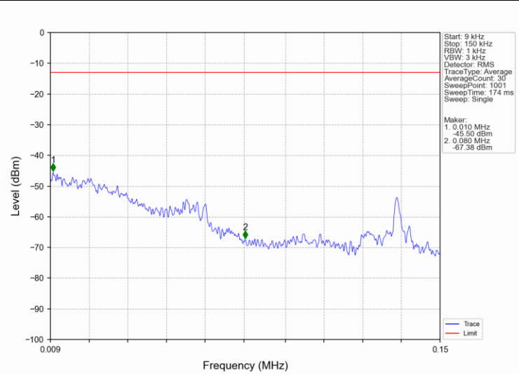
Band5 5MHz 16QAM MCH 836.5MHz RB 1 0 NTNV
