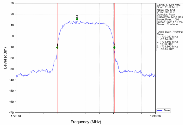
Band4_RMC_MCH_1732.6MHz_12.2kbps_RMC_NTNV
