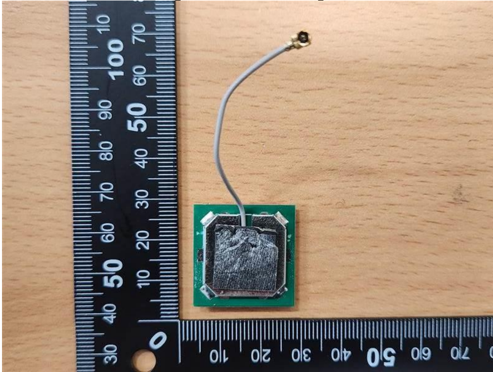
[GPS Antenna 1_without Shield Can]
