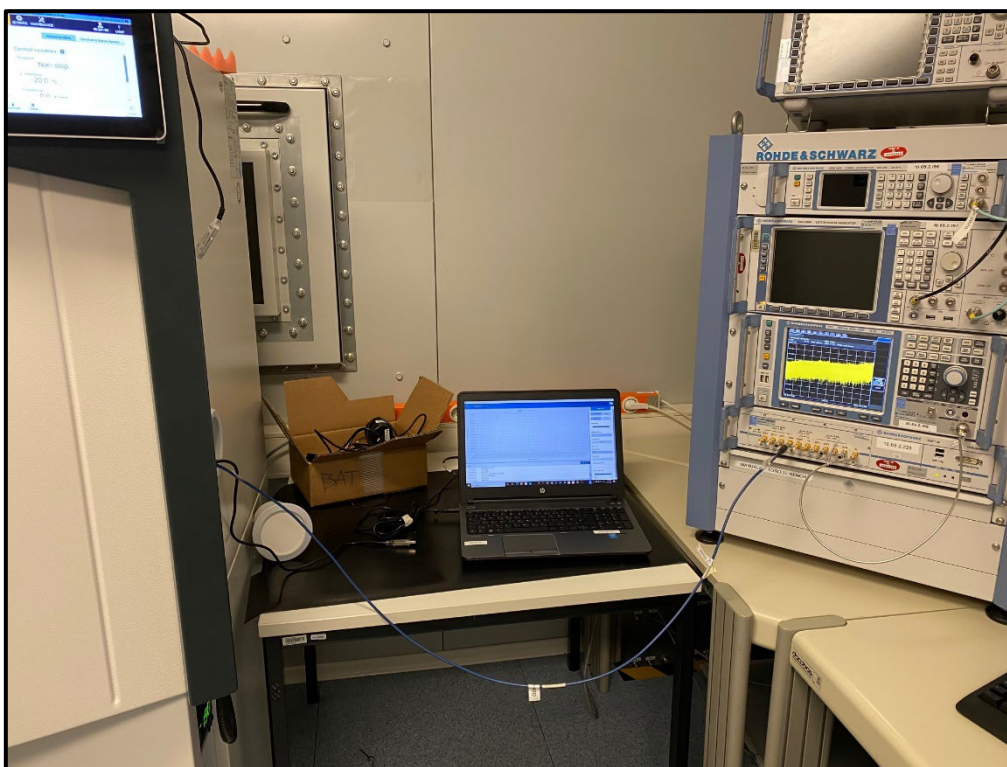
Photo 11: Conducted Test Setup with DC Power Supply
