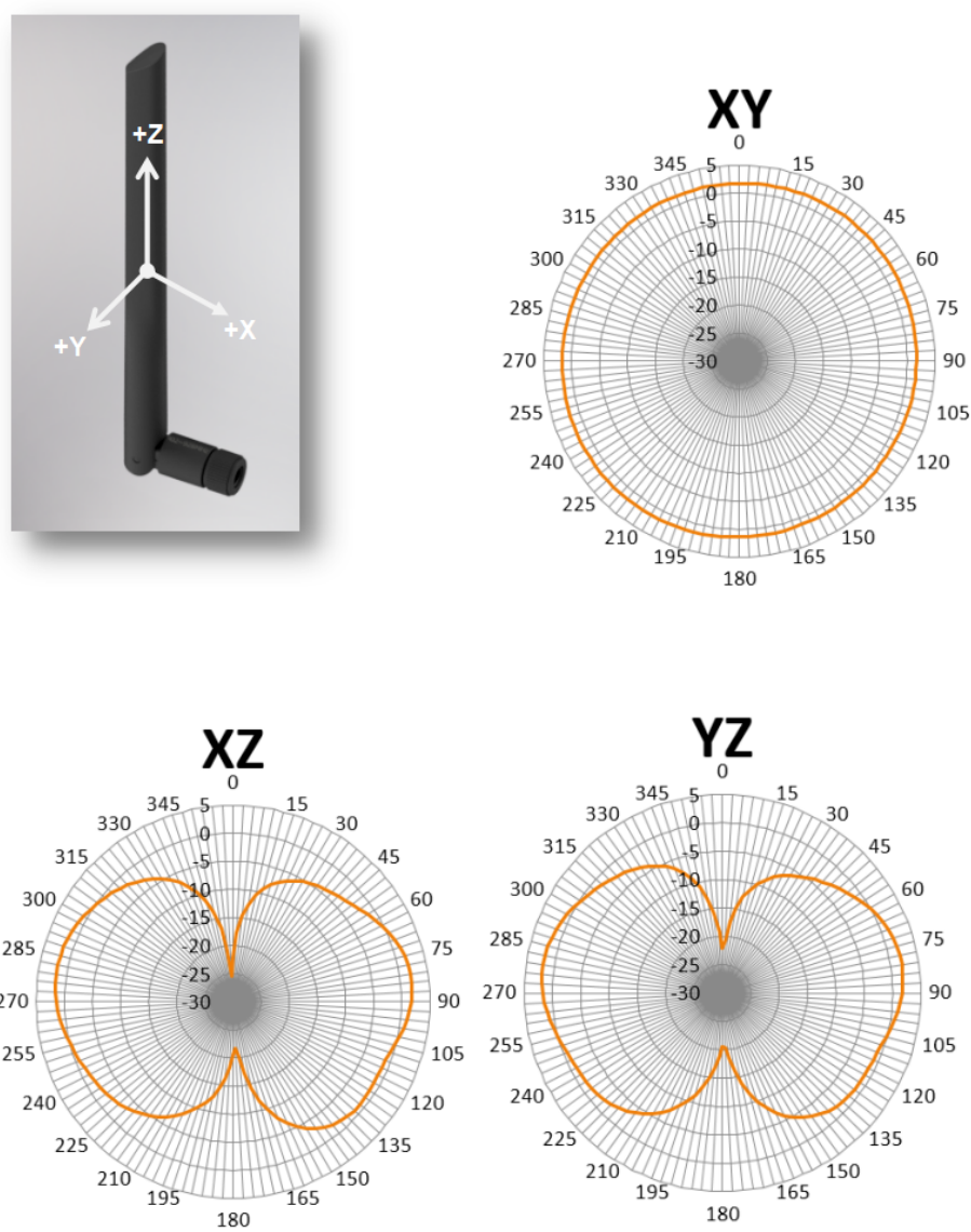
Figure 3: Radiation Patterns
