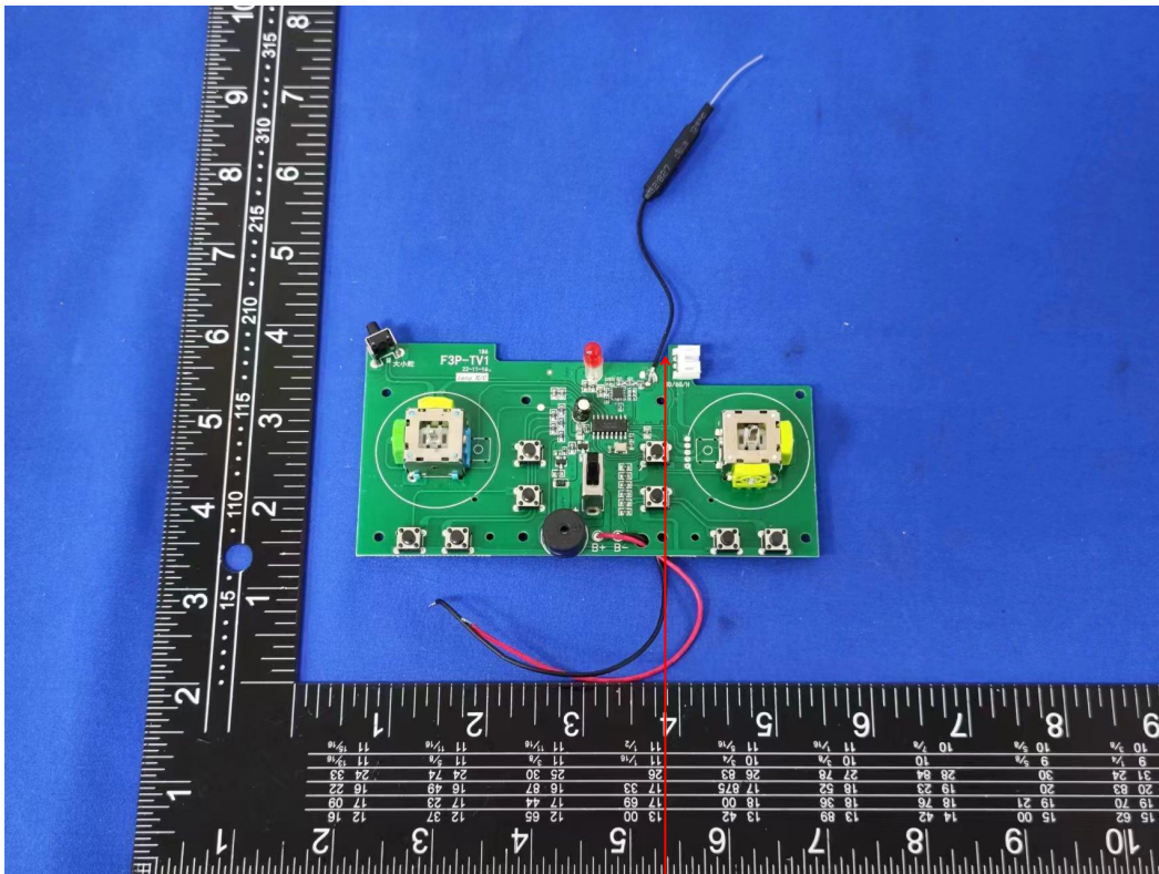
Integral Antenna
