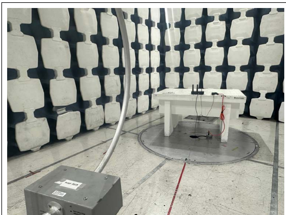
9k-30MHz Front (H4P3-TWC)
