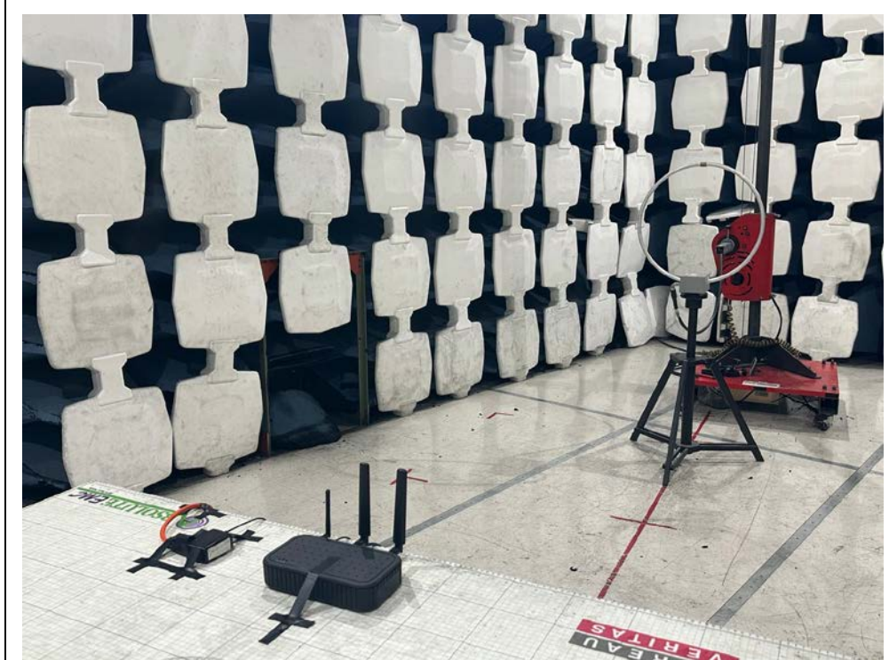
9k-30MHz Rear (H4P3-TWC)
