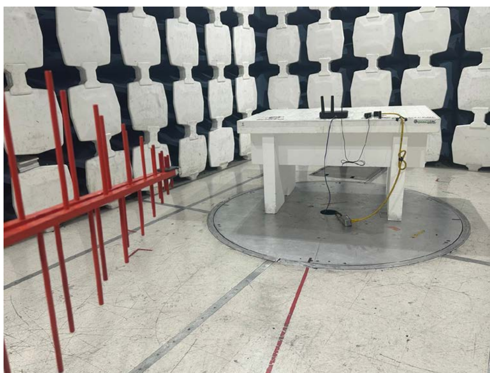
30MHz-1GHz Front (H4P3-TWC)
